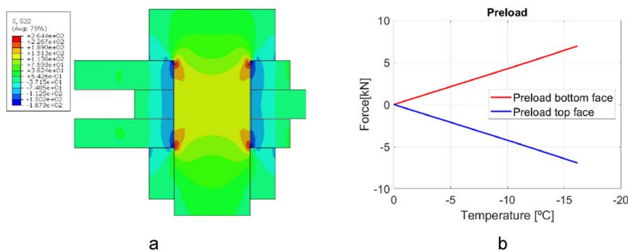
Figure 7. (a) Pressure cone and (b) contact force vs temperature.
