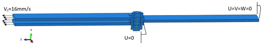
Figure 6. Boundary conditions in the displacement step.
