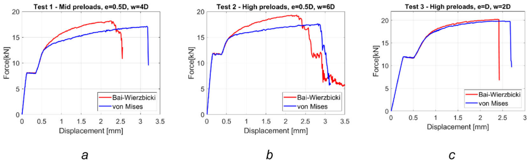
Figure 16. Force displacement curves for additional tests. (a) test 1, (b) test 2, and (c) test 3.
