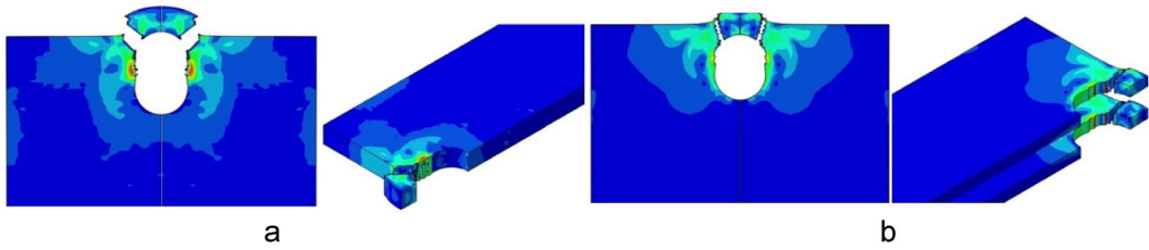
Figure 17. Failure mode observed with (a) Bai-Wierzbicki and (b) von Mises corresponding to width larger than edge distance.
