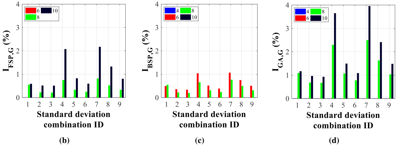
Fig. 12. Comparison of different algorithms for the milling tower. Variation of (a) I_{C,G} , I_{C,FSP} , I_{C,BSP} and I_{C,GA} , (b) I_{FSP,G} ( I_{FSP,G} = 0 for s = 6 ), (c) I_{BSP,G} ( I_{BSP,G} = 0 for s = 4 and 10 ), and (d) I_{GA,G} ( I_{GA,G} = 0 for s = 4 and 6 )
