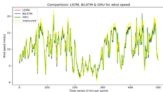
FIGURE 18 Performance comparison: wind speed [43].
