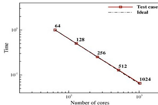
FIGURE 21 Scalability study for turbulent Taylor-Couette flow simulation. The computation time is normalised by the result of 64-processor case [53].
