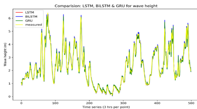
FIGURE 19 Performance comparison: wave height [43].
