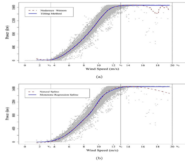
FIGURE 25 Four power curve fitting methods on real data from wind turbines in a wind farm located in Canada: (a) Nadaraya-Watson Kernel Estimator (NWKE) and Tilting Method (TM) applied to NWKE, (b) Natural Cubic Spline (NCS) and Monotone Regression Spline method (MRS) [56].
