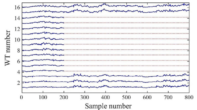
FIGURE 20 An example of wind speed data missing case in large-scale WTs [49].
