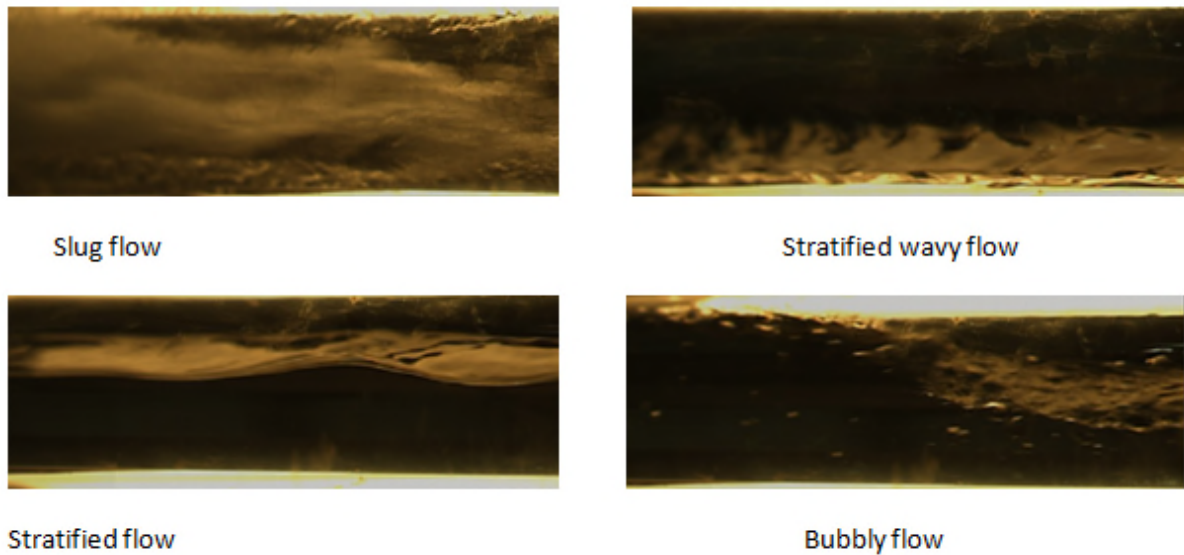
Figure 4-3 Typical flow regimes of the gas-liquid two-phase in a horizontal pipe recorded by a high speed camera
