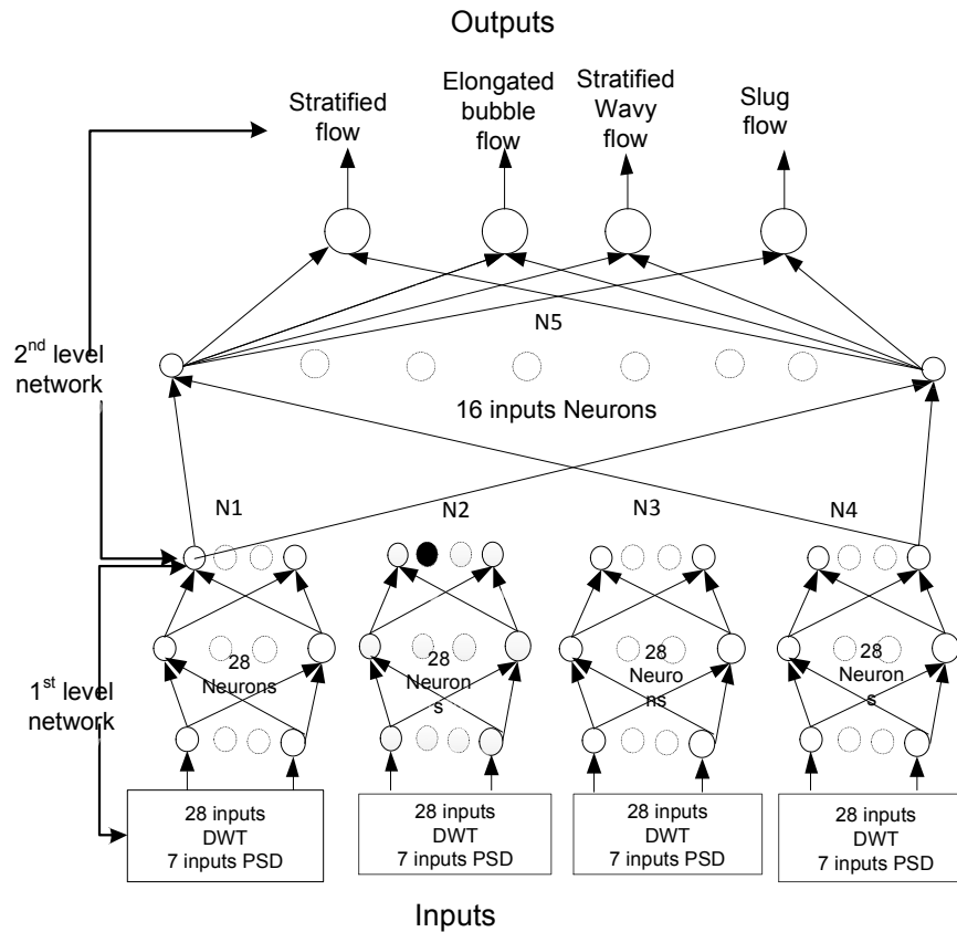
Figure 3-3 A Structure of the flow pattern prediction combined neural network topology (Übeyli and Güler, 2005).
