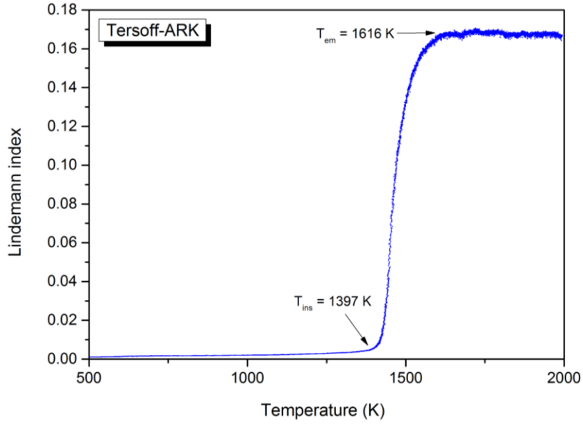
Figure 1: Variation of the Lindemann index upon gradual heating. T_{\text{ins}} corresponds to the phase instability temperature (or first-order melting transition temperature) while T_{\text{em}} corresponds to the bulk molten temperature of silicon.
