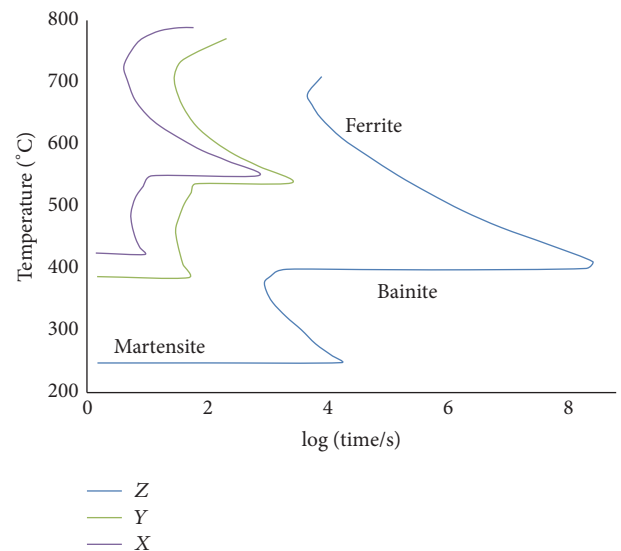
FIGURE 1: Calculated TTT diagrams for steels of composition X (0.15C-0.25Si-0.5Mn-1Mo-2.3Cr wt%), Y (4.3Cr wt%), and Z (9.3Cr wt%) [9–12].
