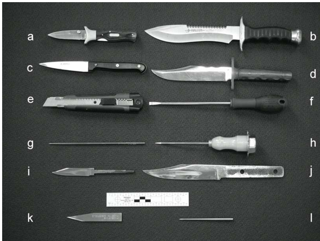
Figure 5. Typical edged weapons a) Lock knife, b) ‘Survival’ knife, c) Kitchen knife, d) ‘Bowie’ knife, e) Craft knife, f) Screwdriver, g) HP White spike (H.P. White 1988), h) American ice pick, i) PSDB N°1 test knife (Parker 1993), j) PSDB N°5 test knife (Parker 1993) , k) HOSDB P1/B test blade (Croft & Longhurst 2007b), l) HOSDB Spike (Croft & Longhurst 2007b).
