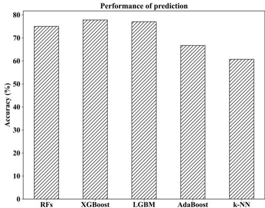
Fig. 18. The accuracy for classifying part density levels of different models.
