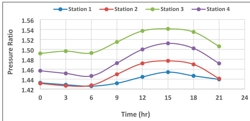
Figure 12. Gas compressor pressure ratio for Scenario 2
