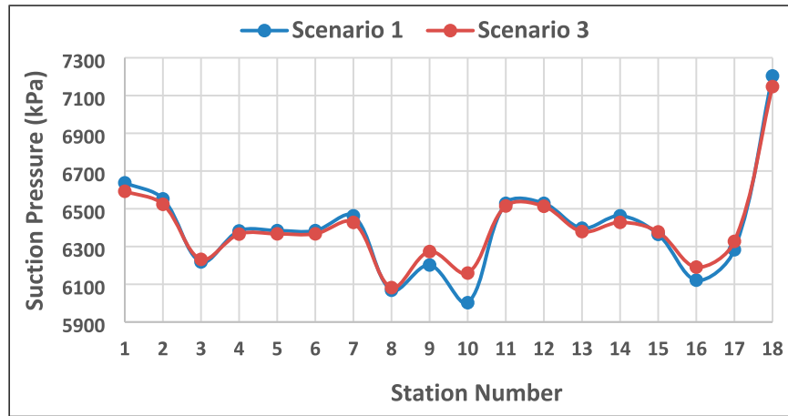
Figure 9. Gas compressor suction pressure for Scenarios 1 and 3
