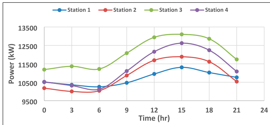
Figure 16. Gas compressor power requirement for Scenario 2
