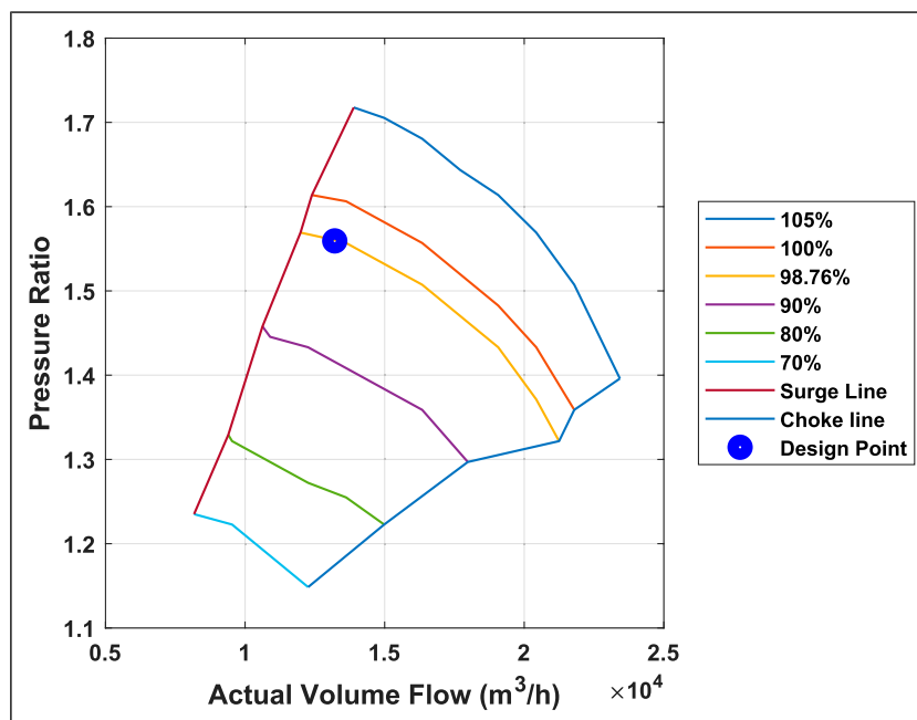
Figure 17. Pressure ratio curve for station 3
