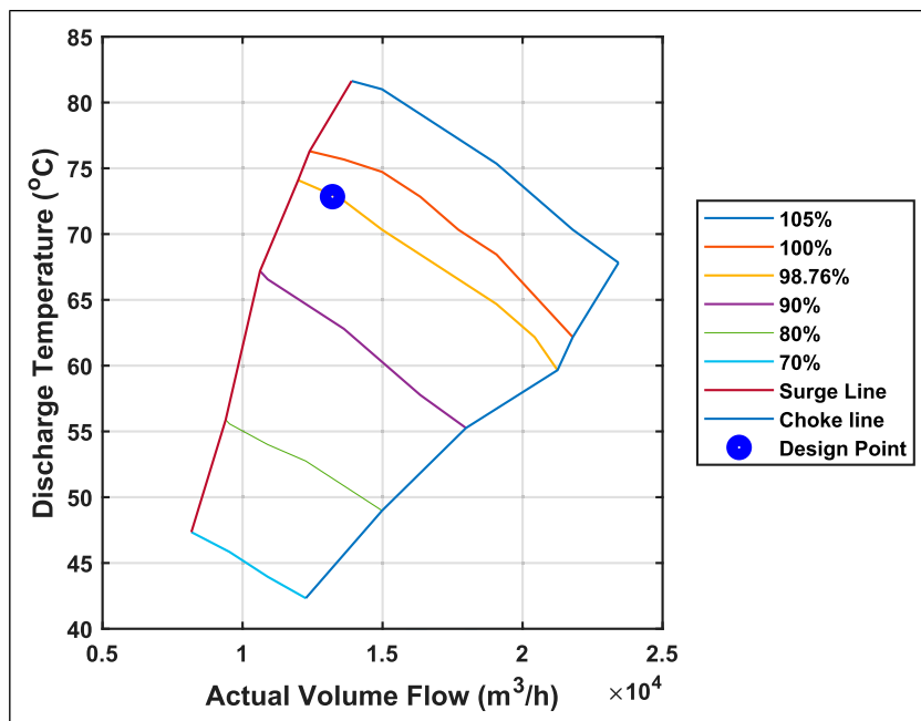
Figure 19. Discharge temperature curve for station 3
