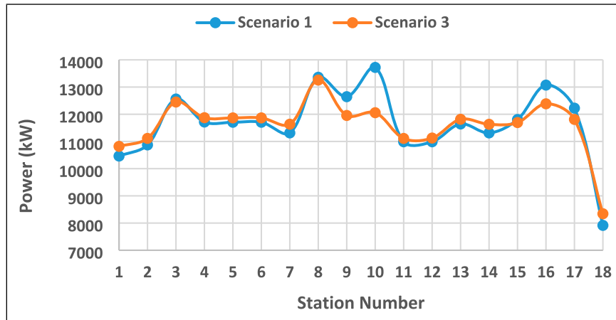
Figure 15. Gas compressor power requirement for Scenarios 1 and 3
