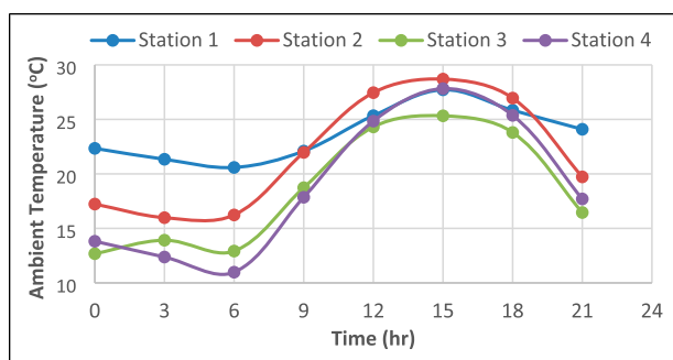
Figure 6. Ambient temperatures recorded at various stations during the winter season.
