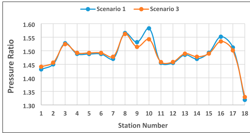
Figure 11. Gas compressor pressure ratio for Scenarios 1 and 3
