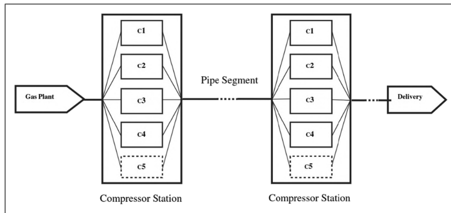
Figure 1. Compressor stations and pipe segments schematic. 31
