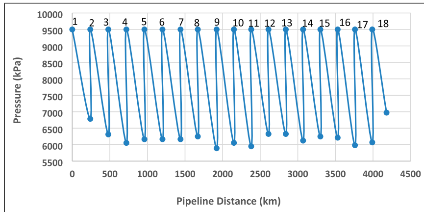
Figure 8. Pipeline pressure drops at various compressor station locations.
