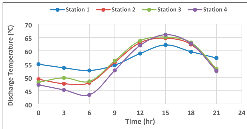
Figure 14. Gas compressor discharge temperature for Scenario 2
