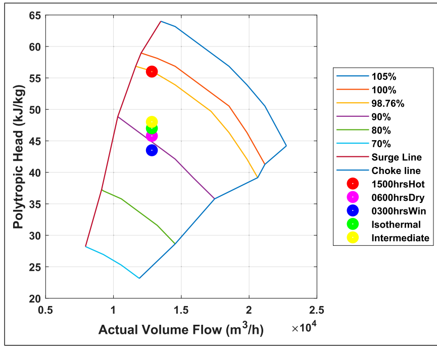
Figure 22. Polytypic head curve for station 2 showing operating points in different flow conditions.
