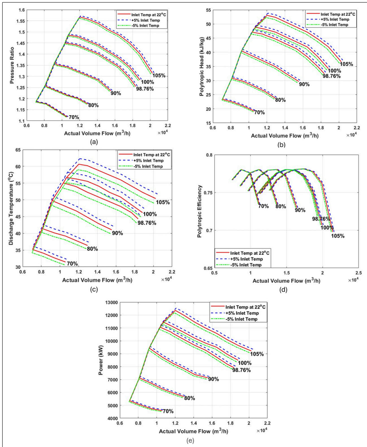
Figure 26. Variation of inlet temperature on compressor (a) pressure ratio (b) polytropic head (c) discharge temperature (d) efficiency (e) power.
