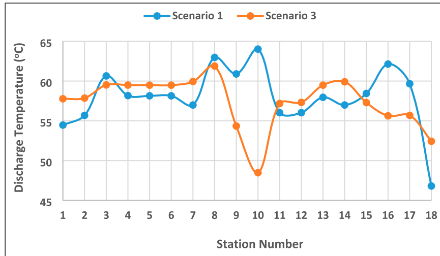
Figure 13. Gas compressor discharge temperature for Scenarios 1 and 3
