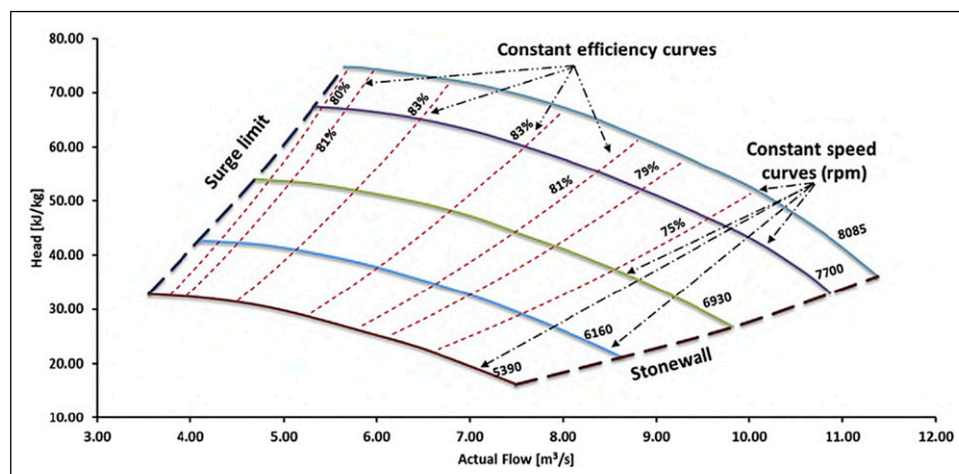
Figure 3. Centrifugal compressor map. 64
