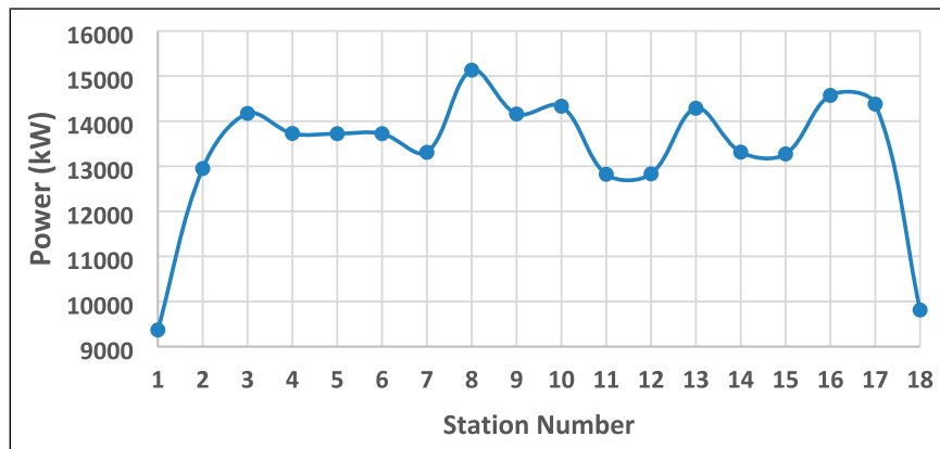
Figure 25. Gas compressor power based on maximum ambient temperature in scenarios 1, 2, and 3
