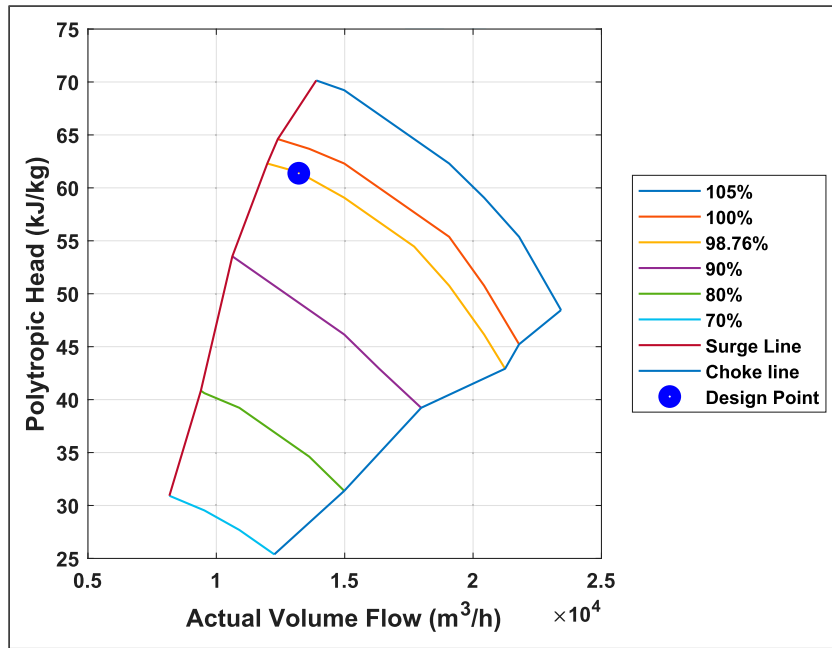
Figure 18. Polytropic head curve for station 3
