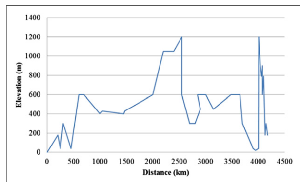
Figure 5. Pipeline elevation-distance profile. 82
