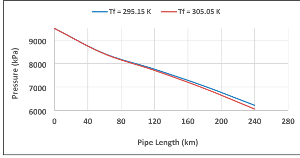
Figure 7. Pressure drops along the pipeline for compressor station 3
