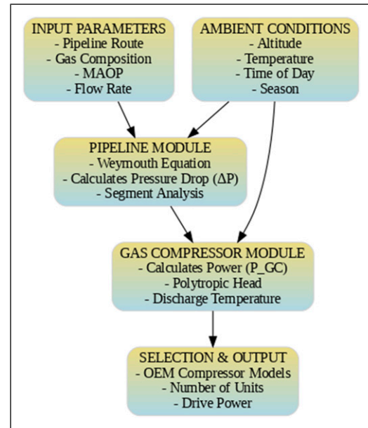
Figure 4. Flowchart of the Techno-Economic and Environmental Risk Analysis (TERA) framework used in the present study. The integrated model processes input parameters through sequential pipeline and compressor modules, conditioned by the ambient data, to produce technical and economic outputs for compressor selection.
