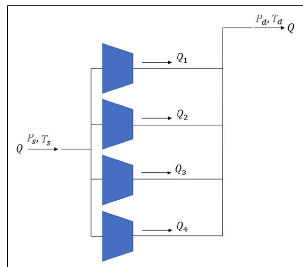
Figure 24. Parallel gas compressors arrangement schematic diagram.
