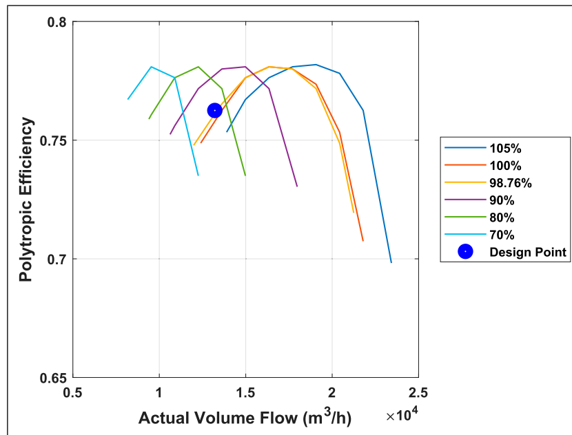
Figure 20. Polytropic efficiency curve for station 3
