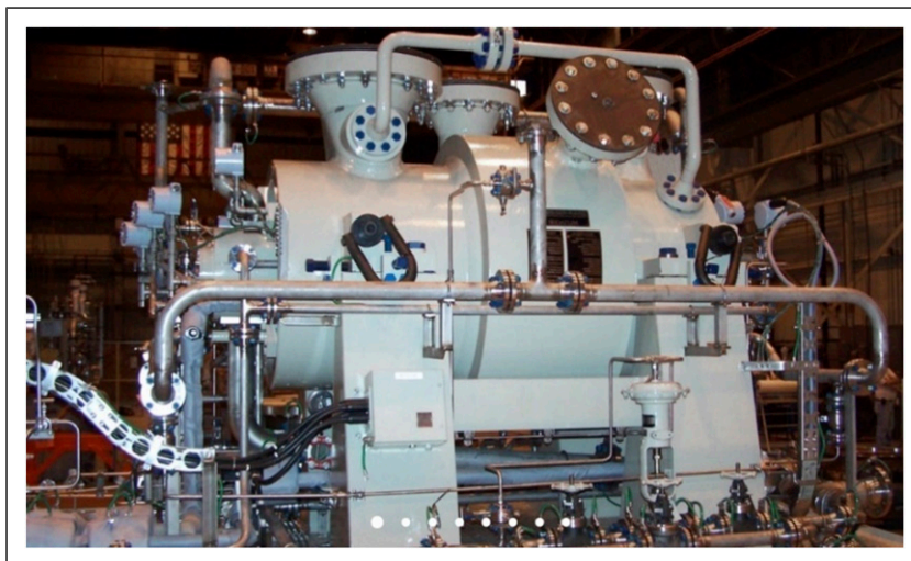
Figure 2. Siemens barrel-type STC-SV compressor. 43
