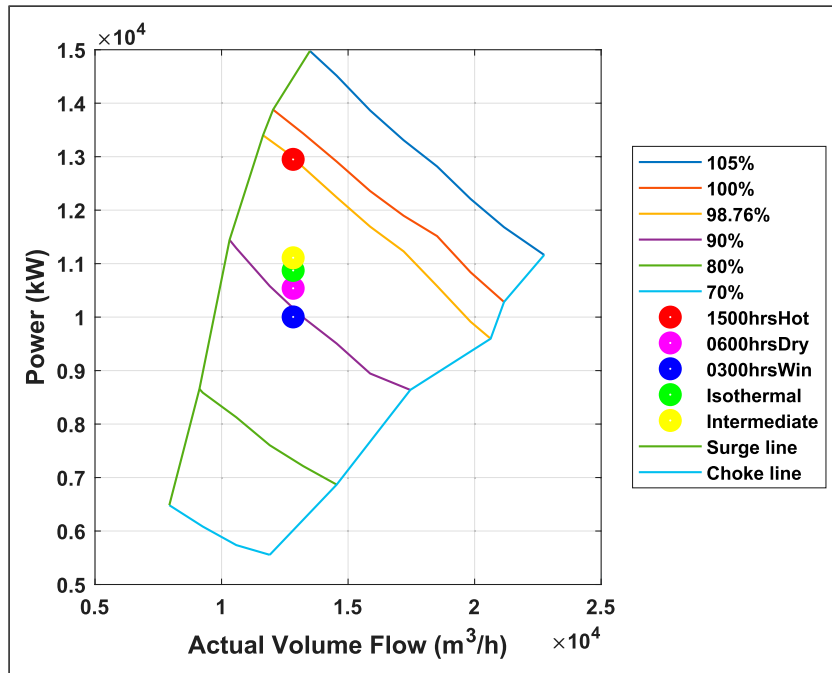
Figure 23. Power curve for station 2 showing operating points in different flow conditions.
