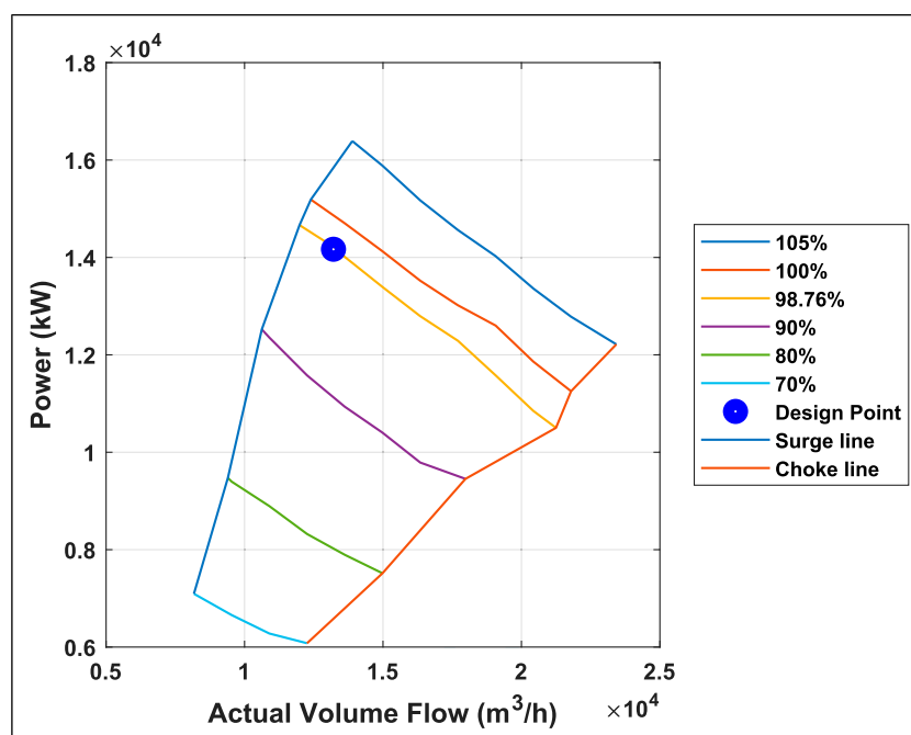
Figure 21. Power curve for station 3
