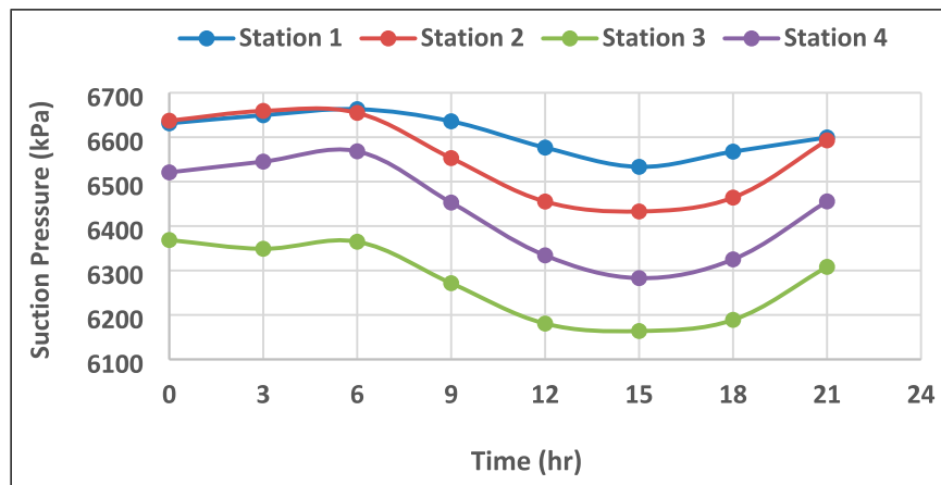
Figure 10. Gas compressor suction pressures for Scenario 2
