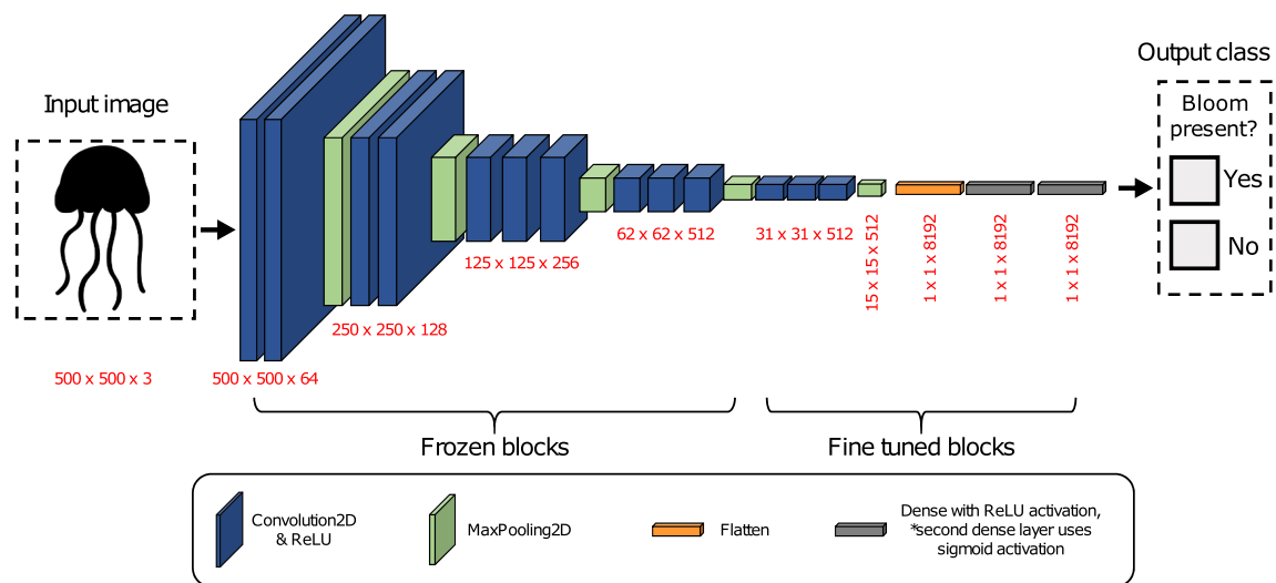
Fig. 4. Model architecture and layers used. An indicative representation of a 500 \times 500 pixel chip's journey from input to prediction. Layer sizes stated in red. ReLU = rectified linear unit.
