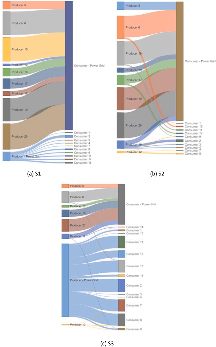
Fig. 6. The supply and demand relationship for 13:00–14:00 in Case 1.
