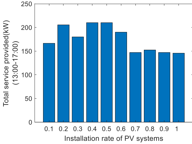
Fig. 18. The total amount of ancillary services provided by the community during 13:00–17:00 given various installation rates of PV systems in Case 6.
