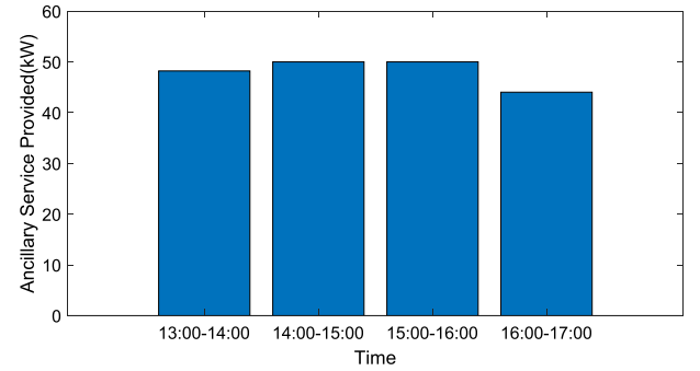
Fig. 11. The total amount of ancillary service provided by the community for 13:00–17:00 in Case 3.
