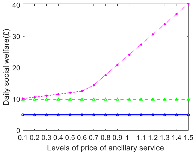
Fig. 13. The social welfare of the residential community given different levels of ancillary service prices in Case 4.
