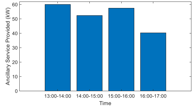
Fig. 10. The total amount of ancillary service provided by the community for 13:00–17:00 in Case 2.
