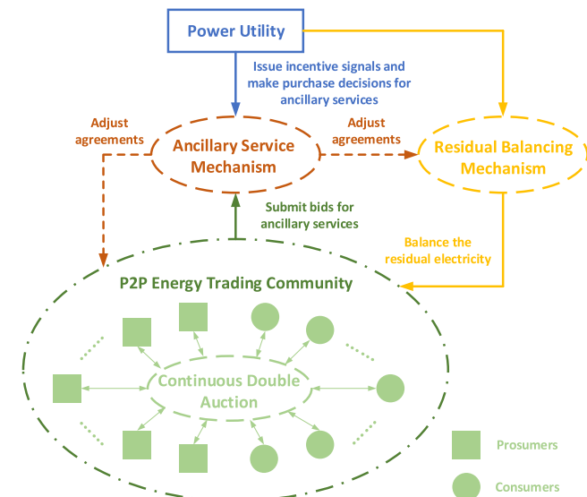
Fig. 1. The methodological framework for ancillary service provision from a P2P energy trading community.
