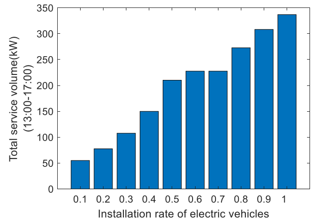
Fig. 16. The total amount of ancillary services provided by the community during 13:00–17:00 given various installation rates of electric vehicles in Case 5.
