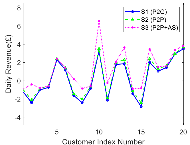
Fig. 4. The revenues of each customer in Case 1.
