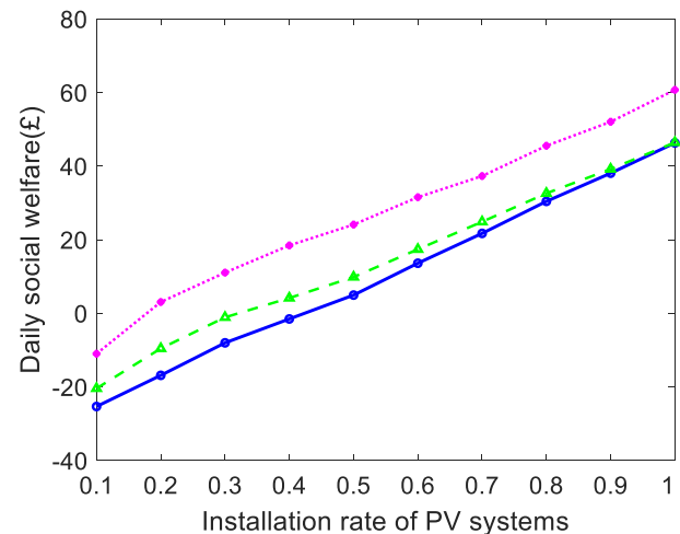
Fig. 17. The social welfare of the residential community given various installation rates of PV systems in Case 6.
