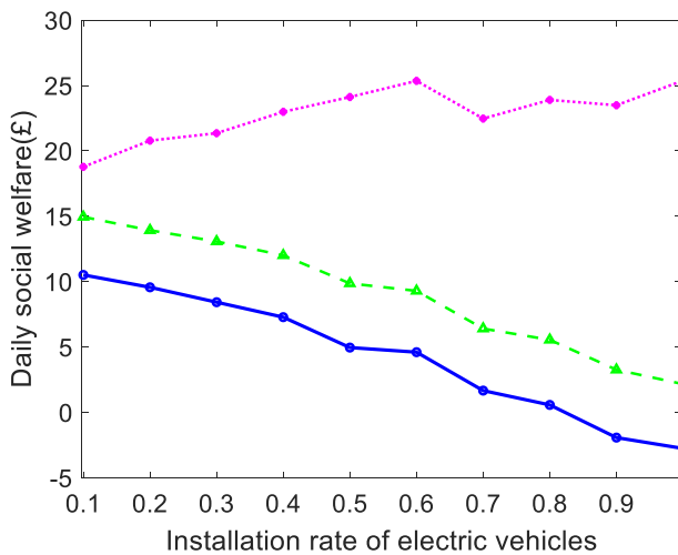
Fig. 15. The social welfare of the residential community given various installation rates of electric vehicles in Case 5.
