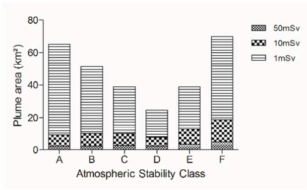
Fig. 2 – Relationship between affected area and atmospheric stability class.
