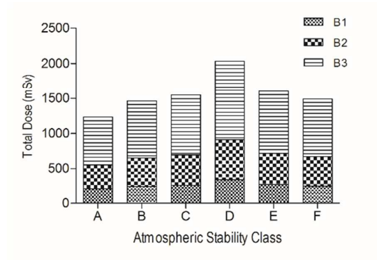
Fig. 5 – Total estimated dose (mSv) at 100 m from hotzone for all subgroups B and for different atmospheric stability classes.
