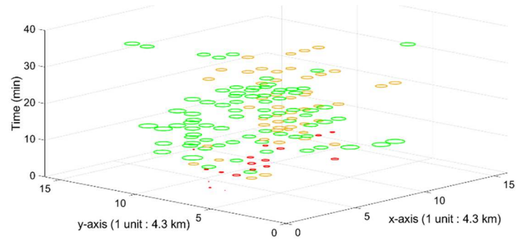
Fig. 6. Safety analysis without weather constraints
