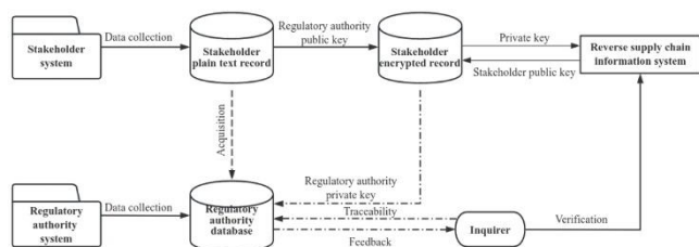
Figure 2. Information security through asymmetric encryption
