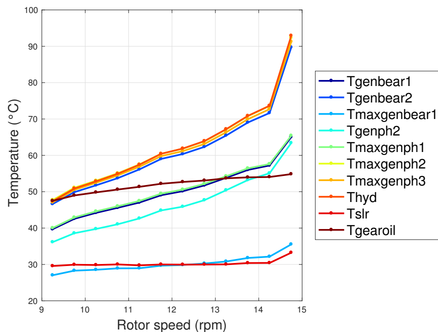
Figure 2. Average curve of the internal temperatures selected by the SVR regression as a function of the rotor speed \omega .
