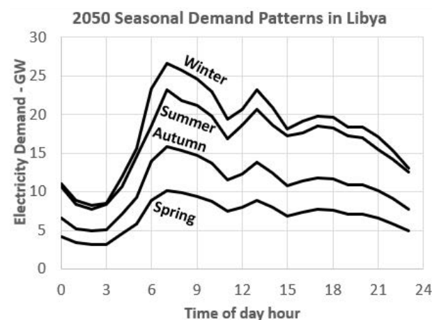
Figure 1. Demand curves for 2050 used in the study.
