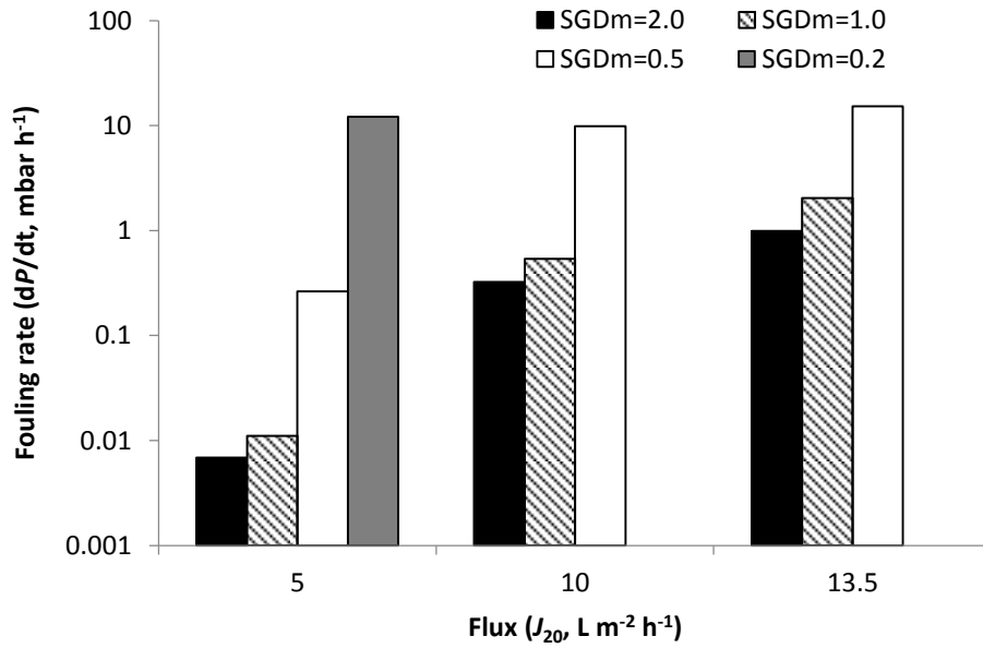
Figure 7. Impact of specific gas demand per unit membrane area ( \text{SGD}_m ) on membrane fouling rate using dead-end gas sparging regime: 9 min on/1 min off; J_{20 \text{ net}}= 5, 10, 13.5 \text{ L m}^{-2} \text{ h}^{-1} . Gas sparging introduced once filtration has stopped. Filtration to 24 h or \text{TMP}_{\max} (550 mbar).
