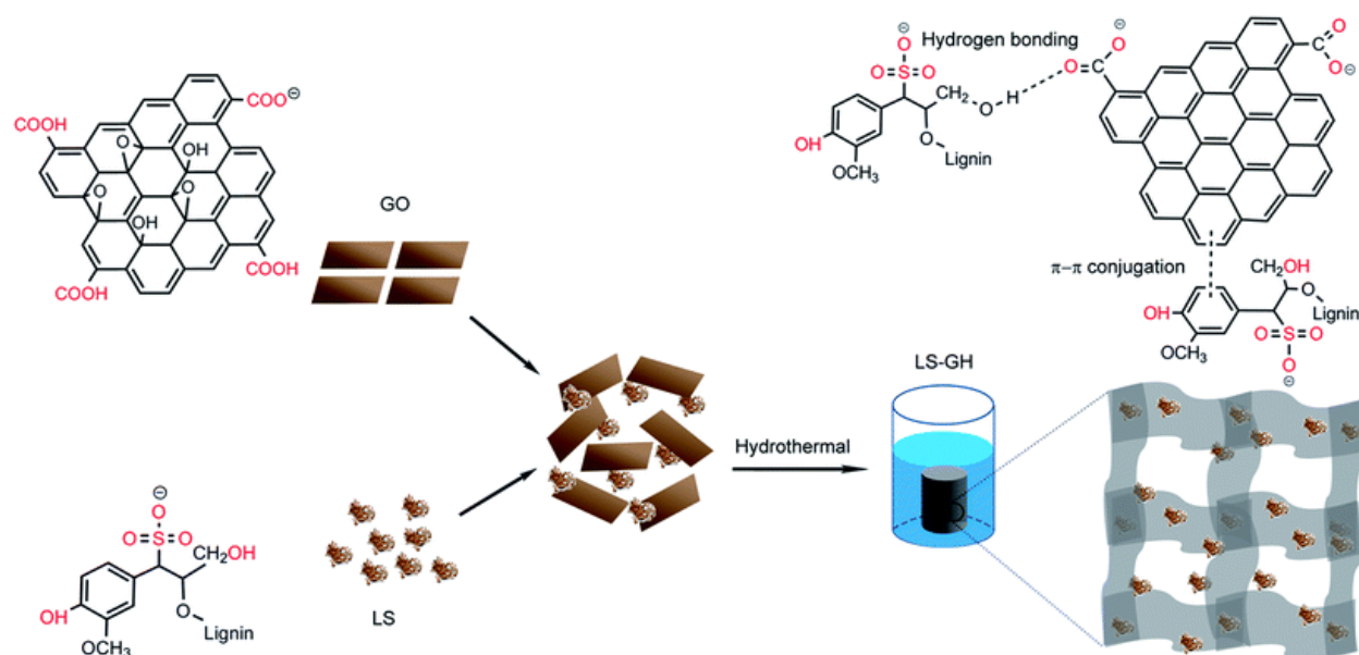
Figure 4. Schematic presentation for the formation of liginosulfonate based graphene hydrogel, hydrogen bonding and pi-pi interactions between reduced graphene oxide and liginosulfonate [88]. Reprinted with permission. [88] Copyright 2016 Royal Society of Chemistry.
