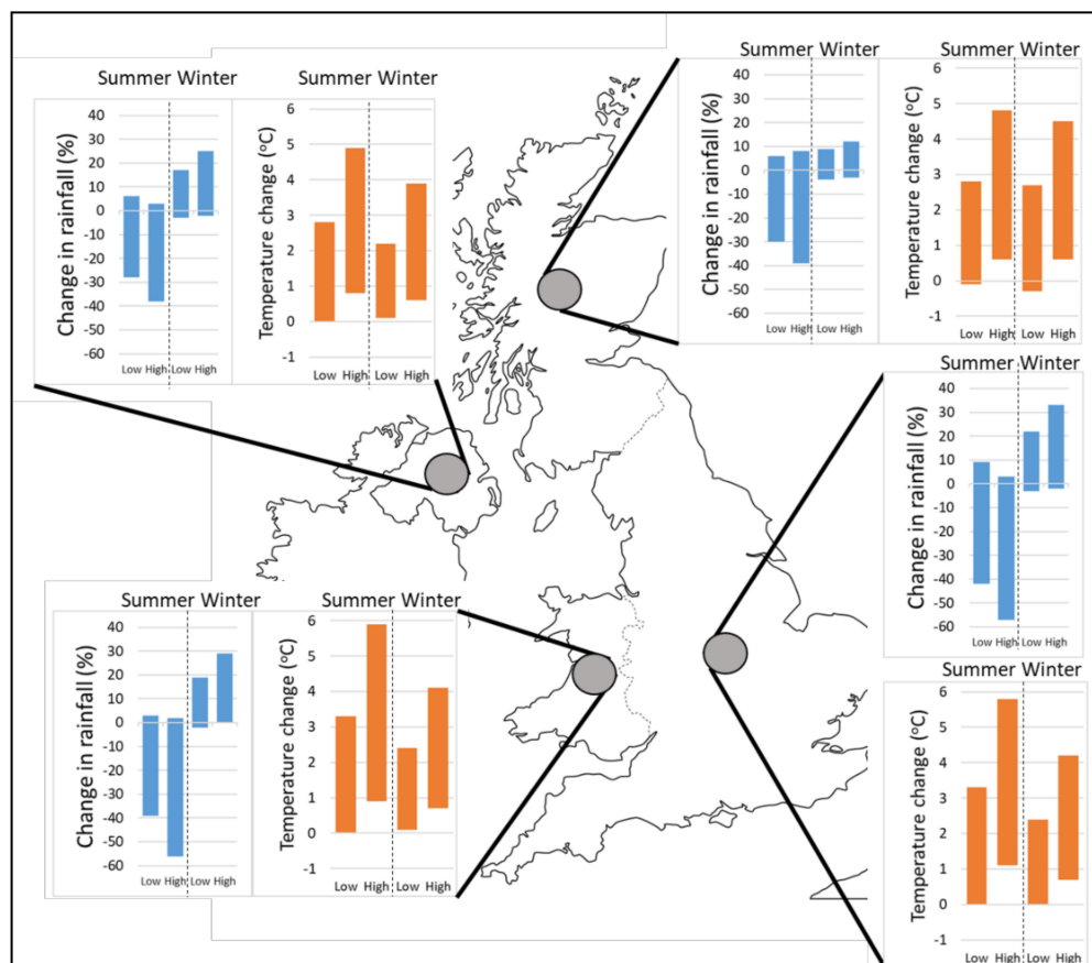
Figure 2. Projected changes in summer and winter rainfall and temperature for indicative central locations in each UK country, from UK Climate Impacts Programme 2018 [7] for High and Low emissions scenarios. All results are for the 10th–90th percentile range for the 2060–2079 period relative to 1981–2000.
