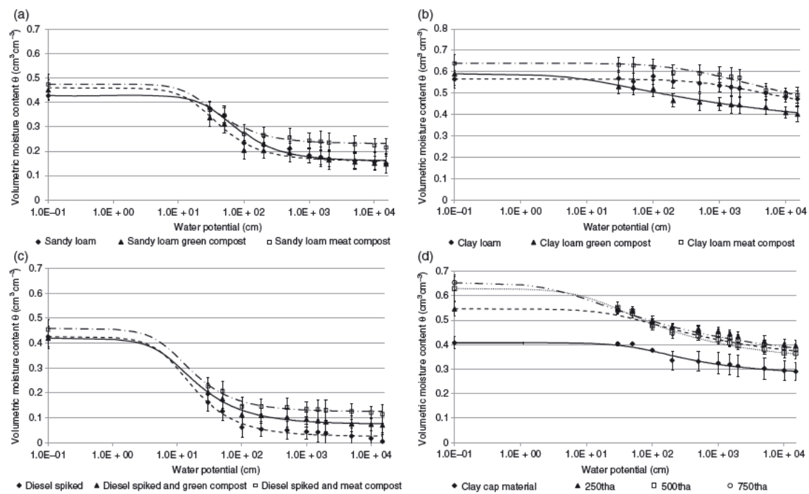
432 433 Fig. 1. Water release curves of unamended and compost amended soils fitted with the Van 434 Genuchten equation: (a) sandy loam; (b) clay loam; (c) diesel spiked sandy loam; (d) field 435 clay cap.
