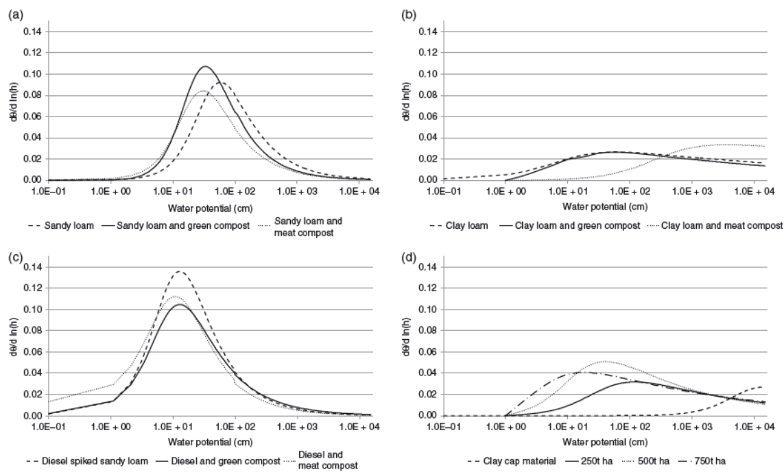
436 437 Fig. 2. Pore size distribution of unamended and compost amended soils represented by the 438 plot of the slope of the release curves against water potential: (a) sandy loam; (b) clay loam; 439 (c) diesel spiked sandy loam; (d) field clay cap.
