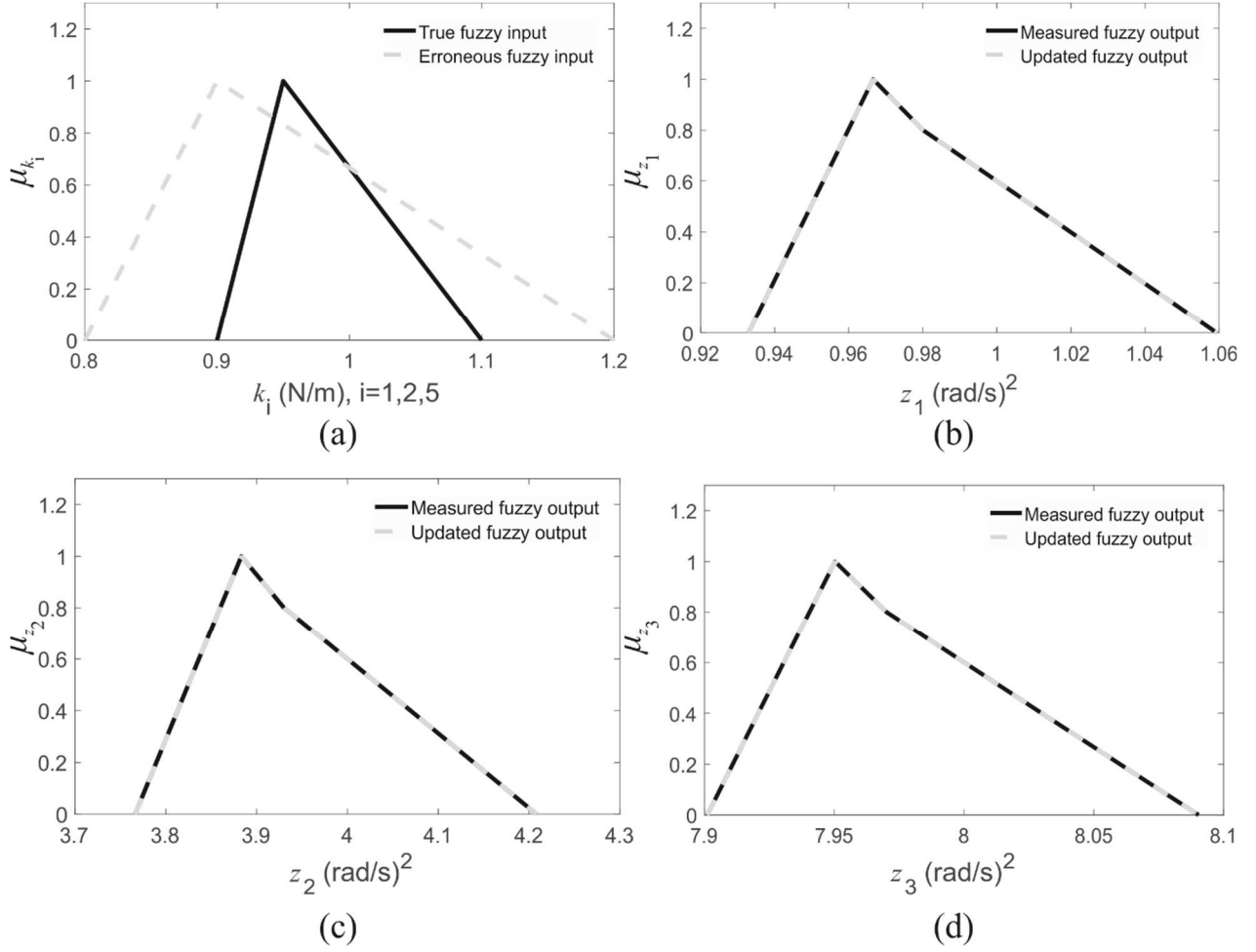
Figure 5: (a) Fuzzy membership functions of the updating parameters (solid: true; dashed: initial), (b) Fuzzy membership functions of the first eigenvalue (solid: measured; dashed: updated), (c) the second eigenvalue (solid: measured; dashed: updated), (d) and the third eigenvalue (solid: measured; dashed: updated) with no measurement noise.
