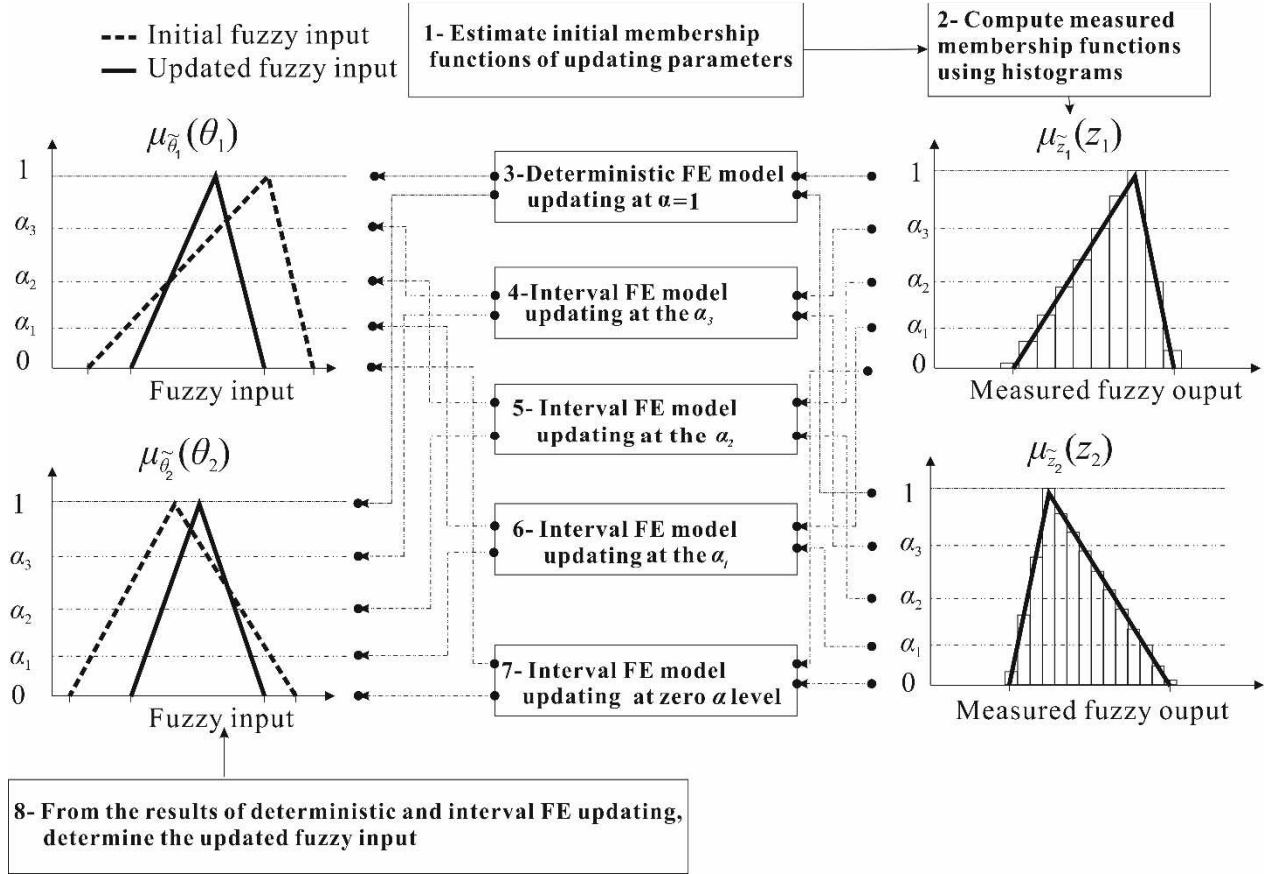
Figure 1: Flowchart for fuzzy finite element model updating using the \alpha -cuts strategy.
