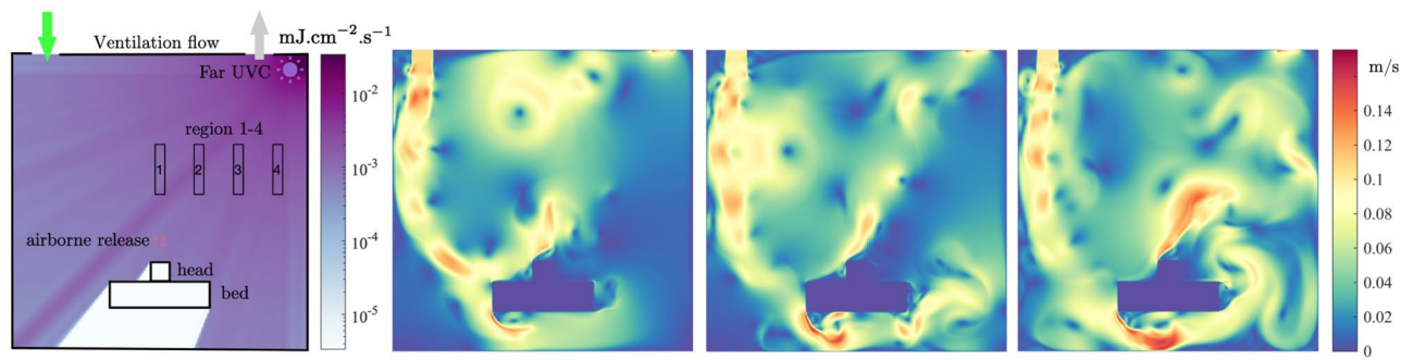
Figure 1. Left to right: Two-dimensional hospital or care home room with bed and patient regions with superimposed far-UVC intensity field (units \text{mJ.cm}^{-2}.\text{s}^{-1} ); Flow velocity profiles at 10, 50 and 100 s following viral release.
