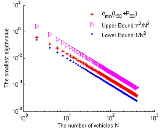
Fig. 5. \sigma_{\min}(L_{BD} + P_{BD}) for BD topology.
