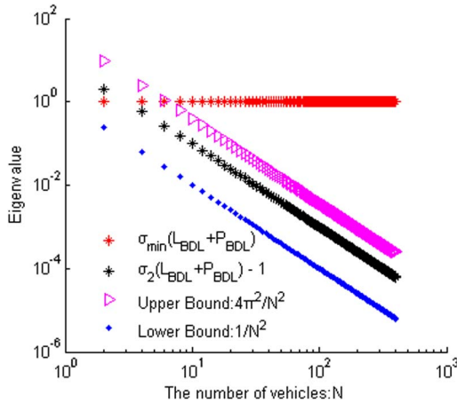
Fig. 6. \sigma_{\min}(L_{BDL} + P_{BDL}) and \sigma_2(L_{BDL} + P_{BDL}) for BDL topology.
