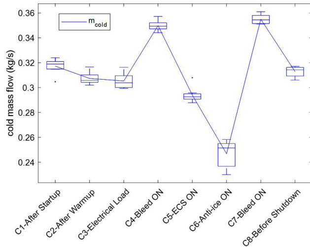
FIGURE 12. Estimated mass flow entering the muffler during various APU operating conditions.
