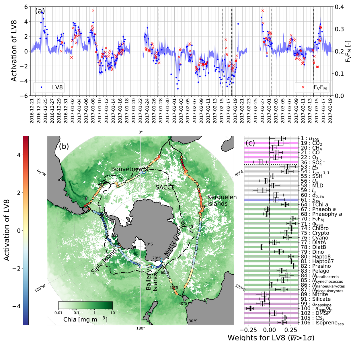
Figure A12. (a) Time series of the activation of LV8 (left axis) and of F_vF_m (right axis). (b) Map of the activation of LV8 and monthly average Chl a concentrations (18 December to 16 January for the Indian ocean sector, 17 January to 17 February for the Pacific sector, and 26 February to 21 March for the Atlantic sector). (c) Weights of the OVs contribution to LV8 for which the bootstrap median was larger than 1\sigma . See the caption of Fig. A1 for details on the oceanic fronts and frontal crossings.
