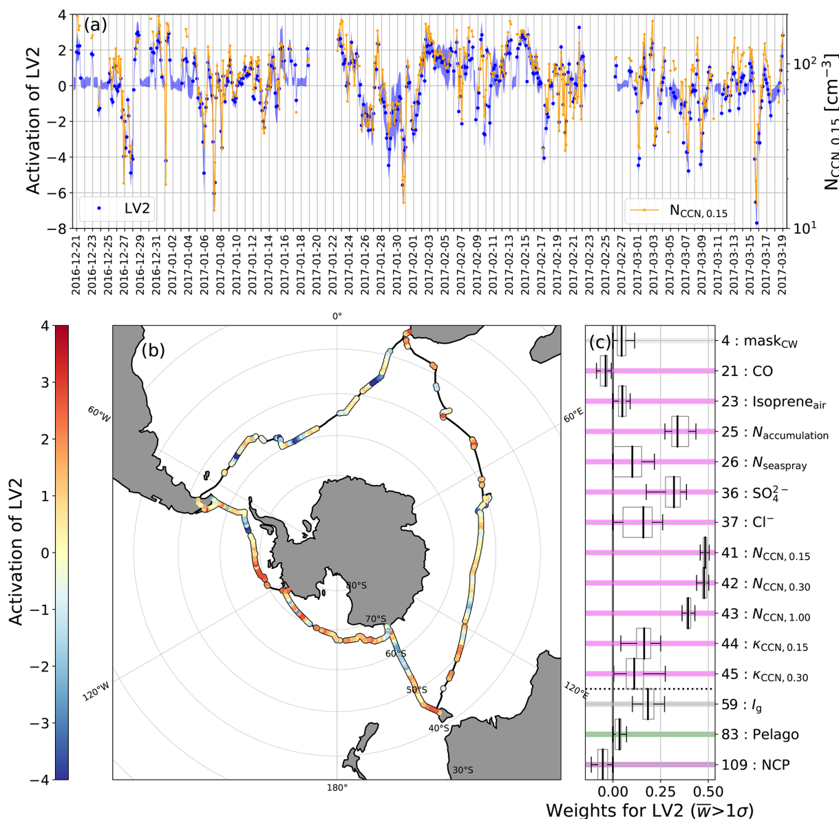
Figure A7. (a) Time series of the activation of LV2 “Drivers of CCN population” (left axis) and of the CCN number concentration at 0.15 % super saturation ( N_{CCN,0.15} , right axis). (b) Map of the ship track coloured by the activation of LV2. (c) Box and whisker plots of the activated weights.
