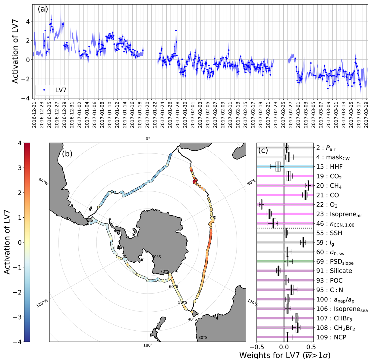
Figure A13. (a) Time series of the activation of LV7. (b) Map of the ship track coloured by the activation of LV7. (c) Box and whisker plots of the activated weights for which the bootstrap median was larger than 1\sigma .
