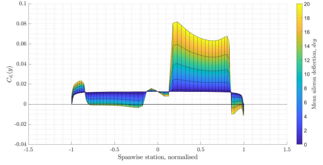
Fig. 5 Elliptic case C_{\delta i}(y) variation with \delta_a .
