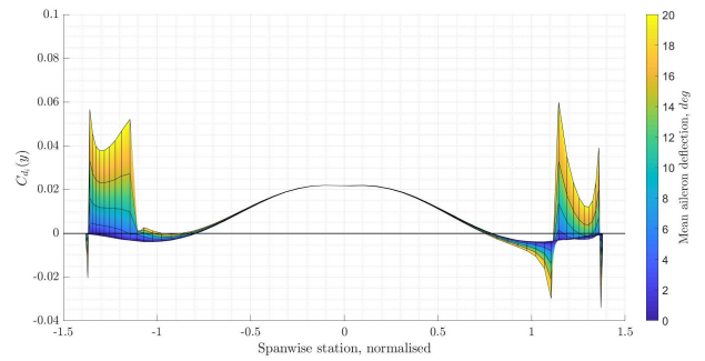
Fig. 7 Cosine case C_{\delta i}(y) variation with \delta_a .
