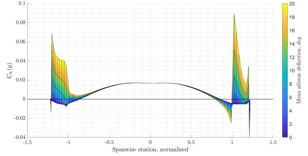
Fig. 6 Prandtl case C_{\delta i}(y) variation with \delta_a .
