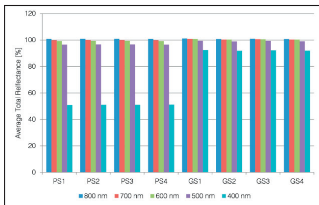
Figure 7. Total Reflectance (contact cleaned)
