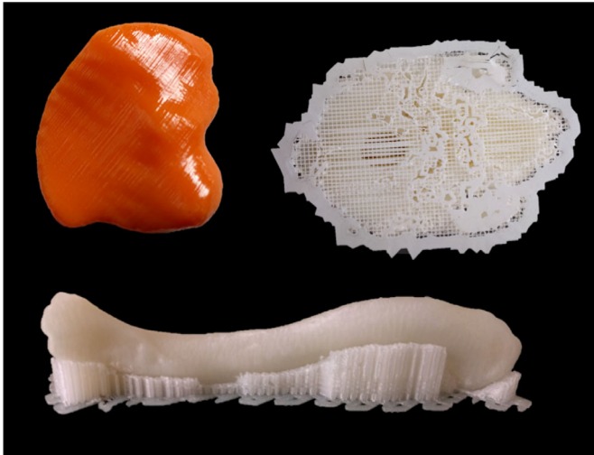
FIG. 5—Photographs of three 3D printed replicas illustrating striations on the surface (upper-left), build raft (upper-right), and support scaffolding (lower). [Color figure can be viewed at wileyonlinelibrary.com ]
