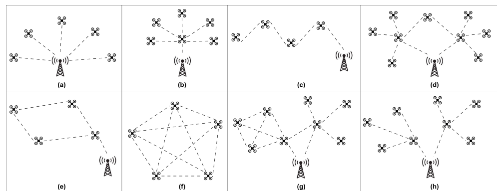
Figure 3. FANET architectural classification: (a) centralised single hop, (b) leader–follower star, (c) multi-hop relay, (d) clustered hierarchical, (e) single-layer cluster, (f) peer-to-peer mesh, (g) hybrid, and (h) centralised star.
