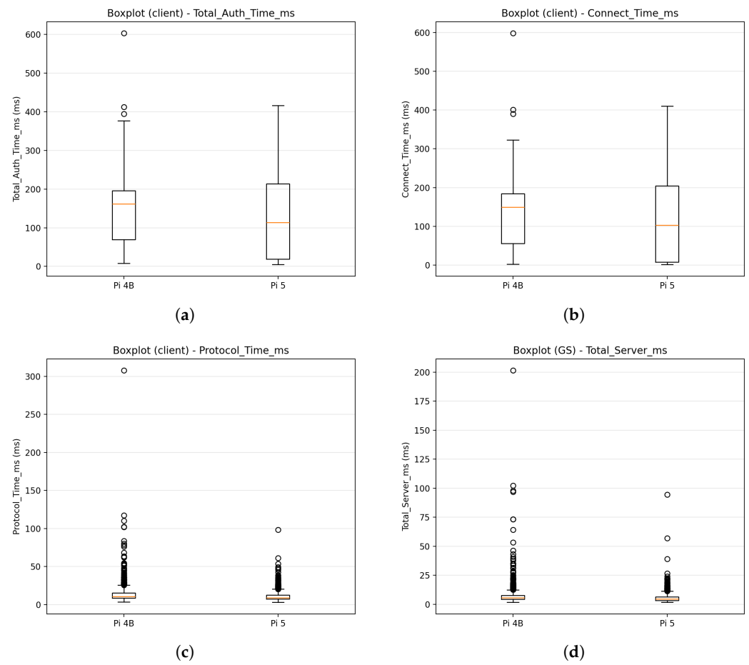
Figure 9. Boxplot comparison (Pi 4B vs Pi 5) for client- and server-side latency metrics over successful sessions ( n = 3000 per platform). (a) Total_Auth_Time_ms (UAV); (b) Connect_Time_ms (UAV); (c) Protocol_Time_ms (UAV); (d) Total_Server_ms (GS).
