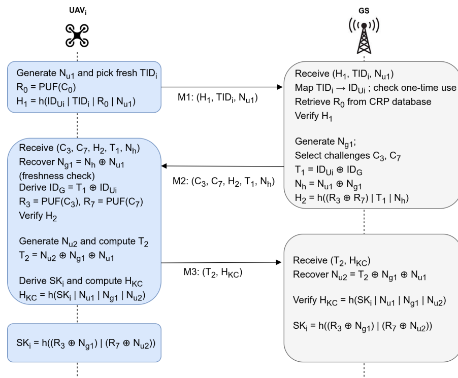
Figure 4. Message flow of the proposed three-message UAV-GS mutual authentication protocol.
