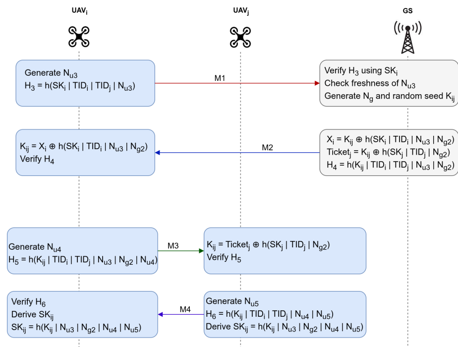
Figure 5. UAV-UAV session key establishment.
