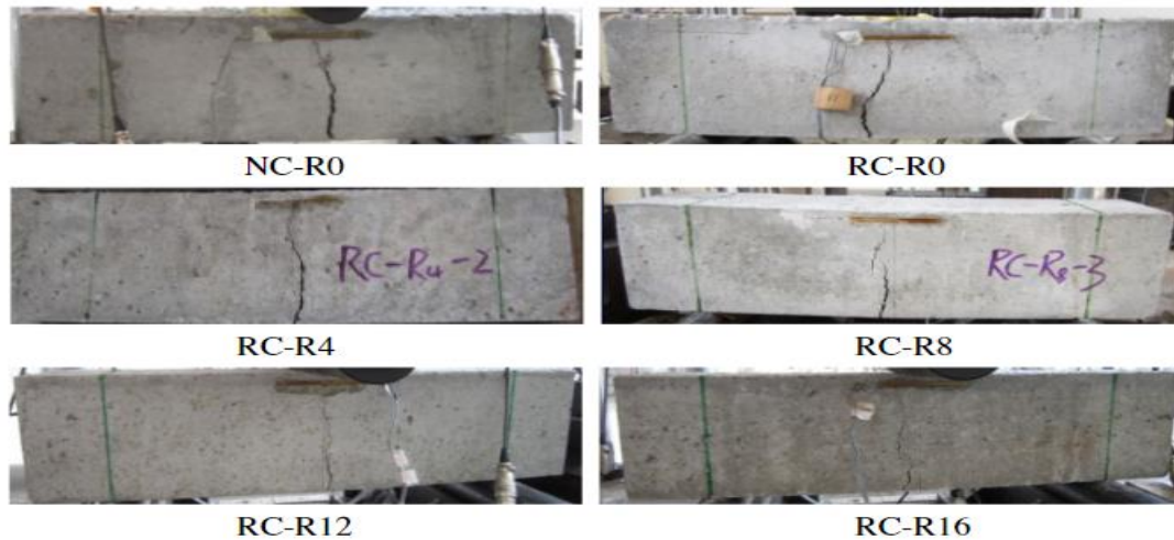
Figure-7 Flexural failure modes of rubber crumb and SF-reinforced RAC [123].
