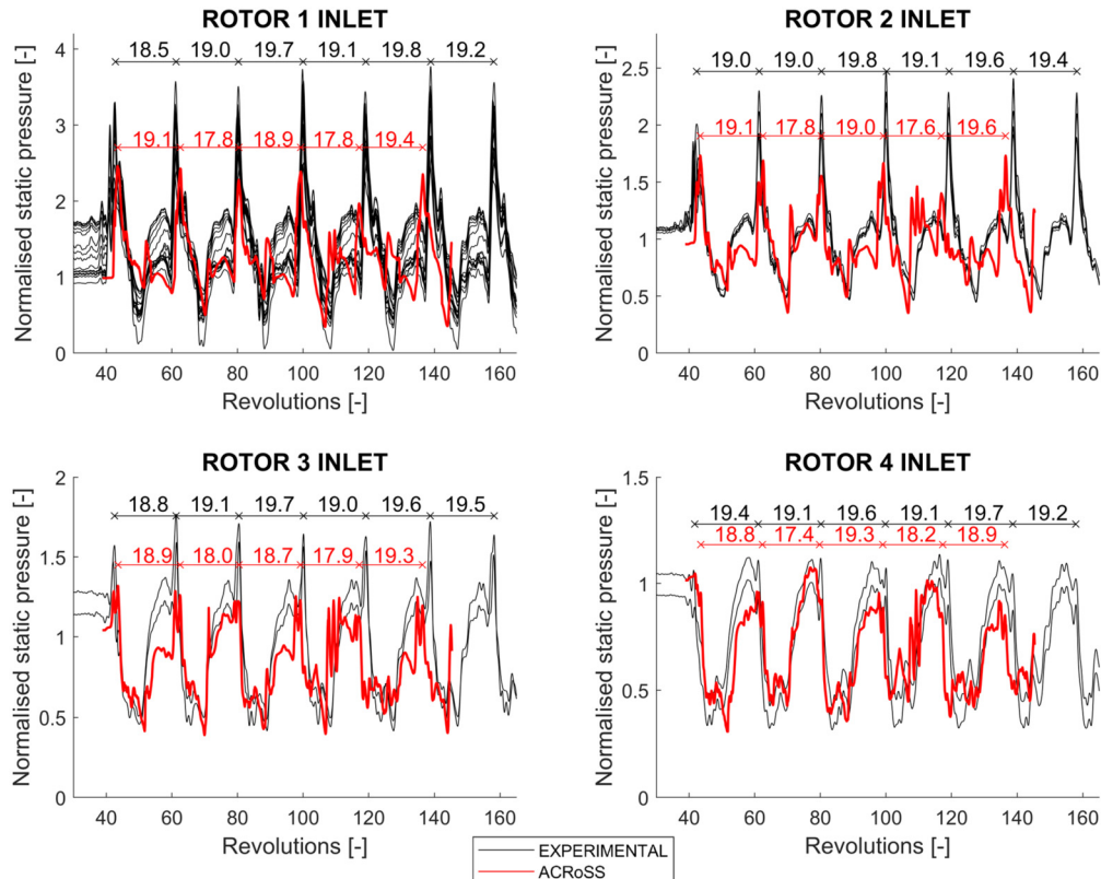
Fig. 9. Static pressure at each rotor inlet tip, comparison of experimental data and ACroSS simulations, with choked nozzle. Case 1 minimum volume.
