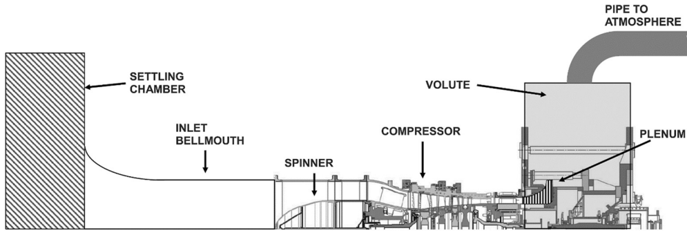
Fig. 2. The DLR Rig 250 test facility, including original image from Giersch et al. [3]. Not in scale.
