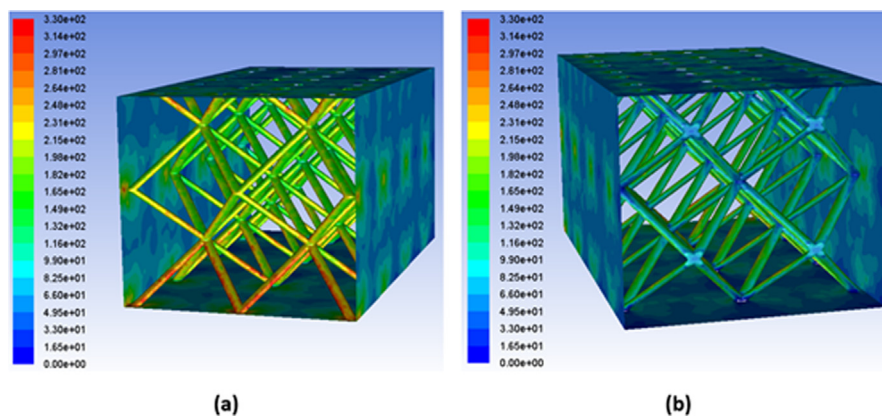
Fig. 16. Local heat transfer coefficient ( \text{W/m}^2 \cdot \text{K} ): inlet view (a), outlet view (b).
