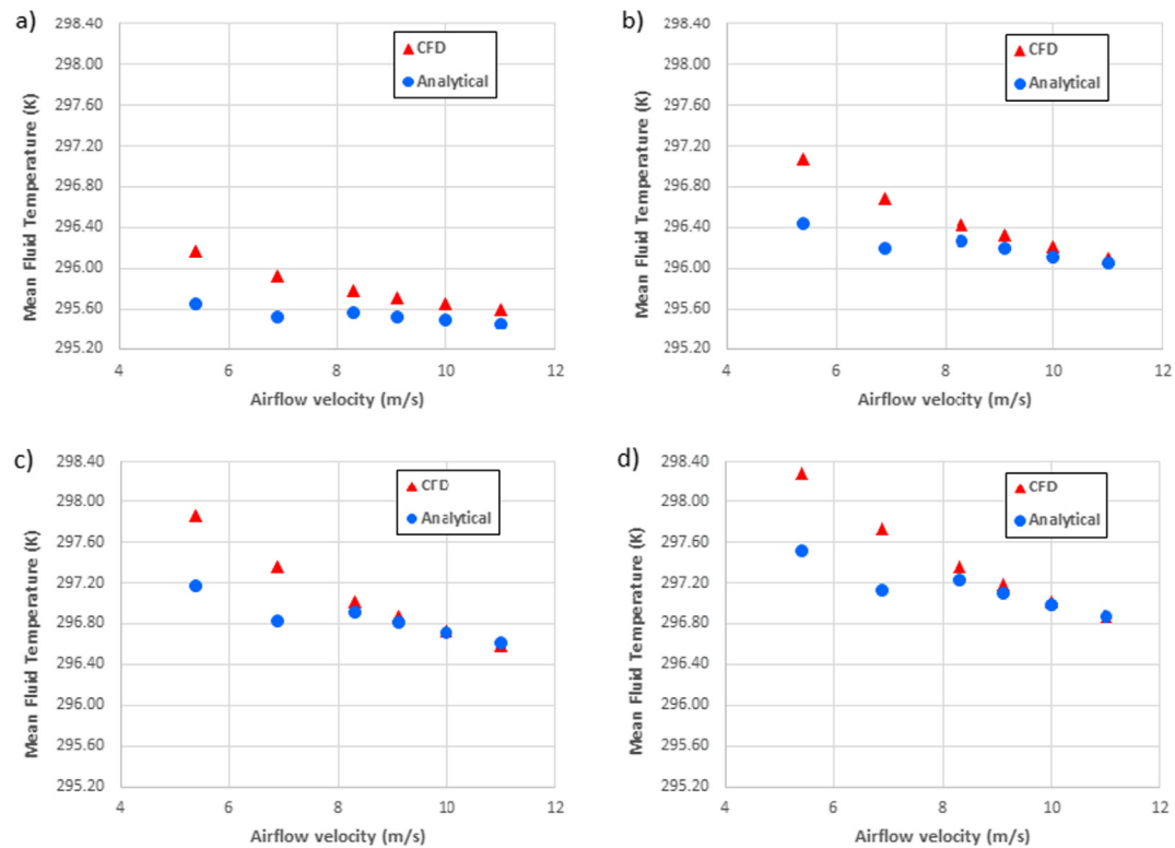
Fig. 12. Comparison between analytical and numerical mean fluid temperatures of Planes n° 1 (a), 2 (b), 3 (c) and 4 (d) with respect to u_0 for T_w = 320 K and T_0 = 294.8 K.
