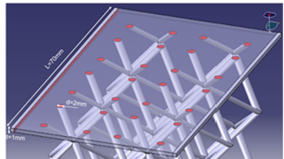
Fig. 4. Contact surfaces with top wall.
