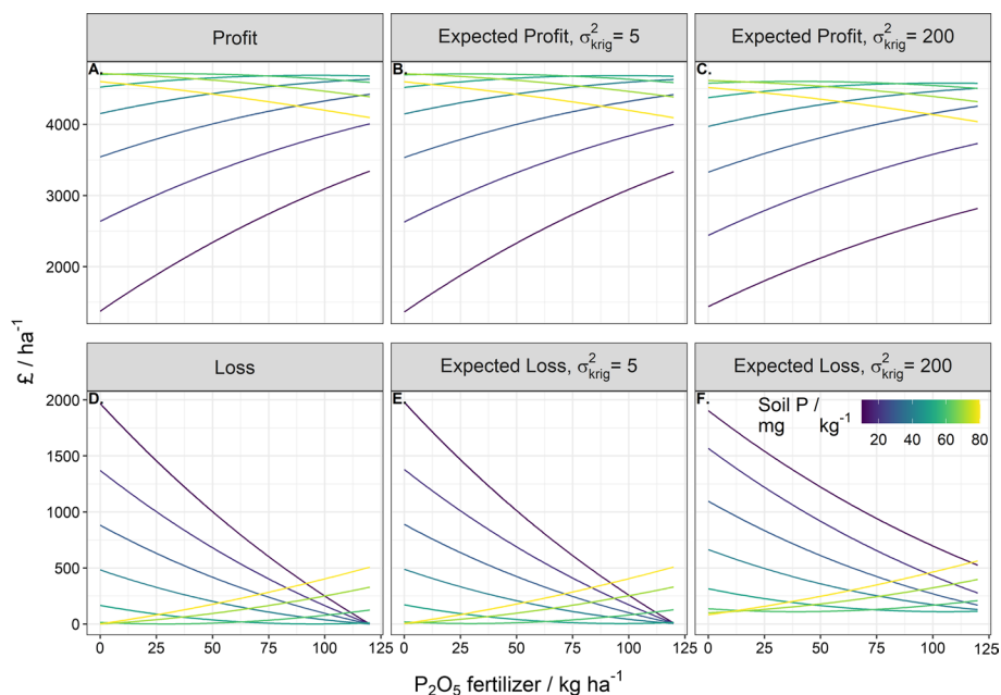
Fig. 3 Profit and loss under zero error variance, expected profit and loss under an error variance of 5 \text{mg kg}^{-1} and an error variance of 200 \text{mg kg}^{-1} for a range of estimated soil P values from 10 to 80 \text{mg kg}^{-1} . The range of P fertiliser applied spans 0 to 120 \text{kg ha}^{-1}
