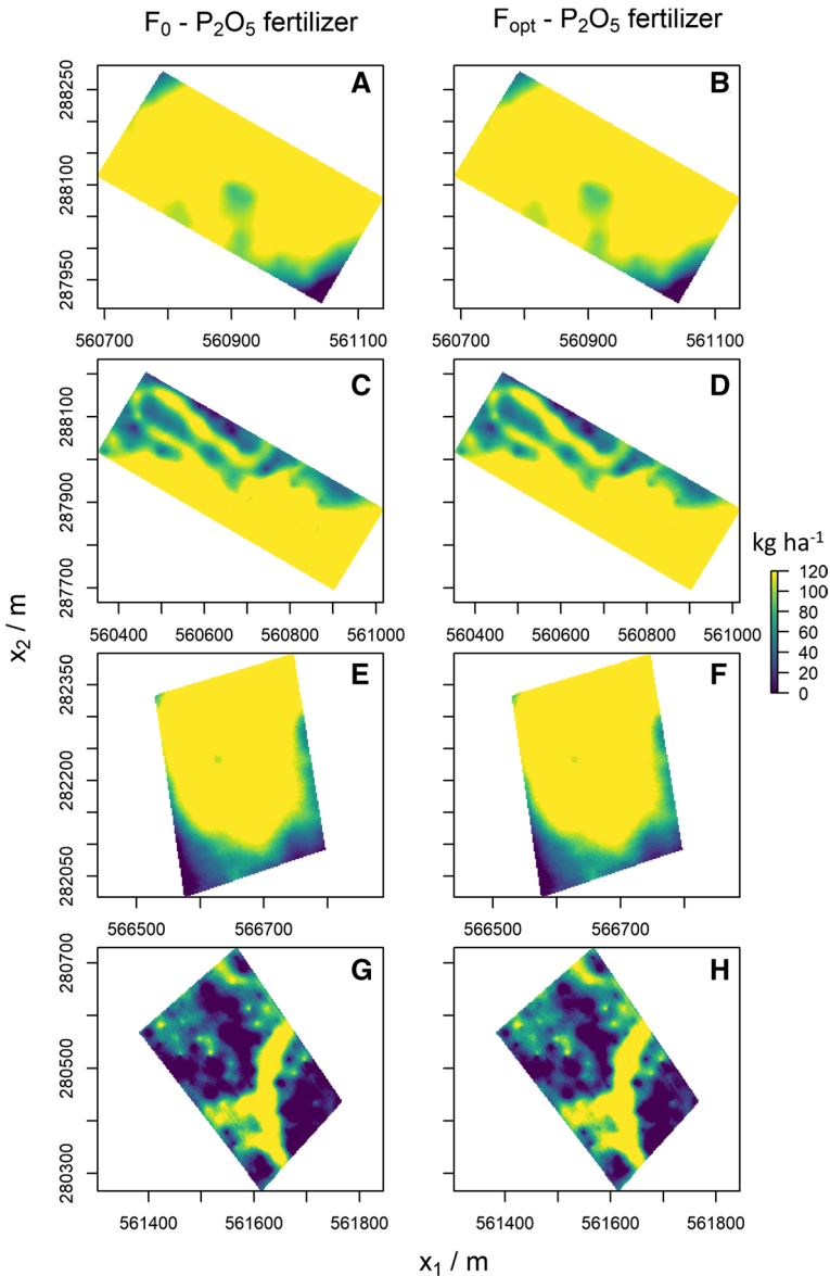
Fig. 5 Optimum P fertiliser application with perfect knowledge of soil P ( F_0 ), optimum application when accounting for \sigma_{\text{krig}}^2 in the estimate of soil P ( F_{\text{opt}} )
