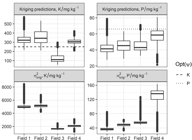
Fig. 7 Box-plots of kriging predictions and the kriging variance ( \sigma^2_{\text{krig}} ), by field for available P and K, horizontal lines represent the nutrient value for which the maximum yield, \text{Opt}(\psi) , is obtained on the fitted dose–response curve
