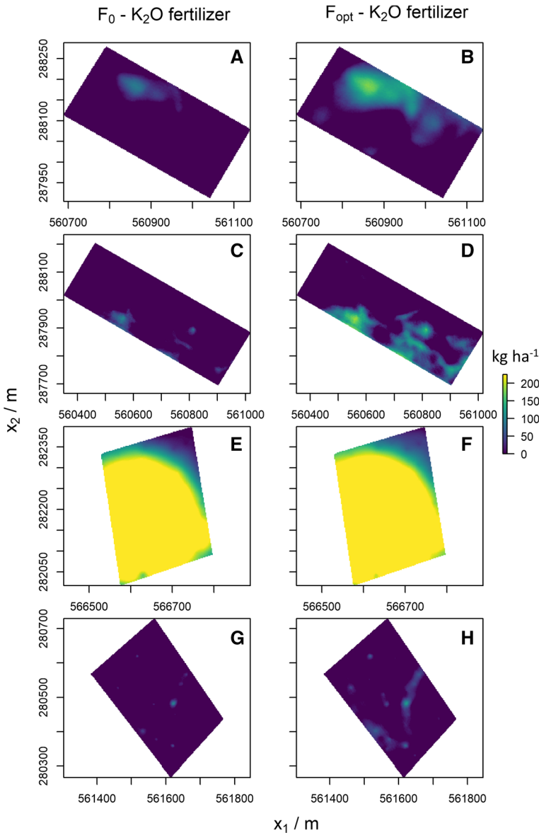
Fig. 6 Optimum K fertiliser application with perfect knowledge of soil K ( F_0 ), optimum application when accounting for \sigma_{\text{krig}}^2 in the estimate of soil K ( F_{\text{opt}} )
