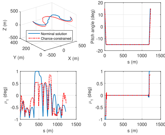
Fig. 11: Nominal and chance-constrained results
