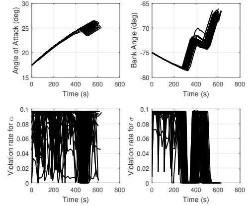
Fig. 9: 500 evolutions of the control and constraint results
