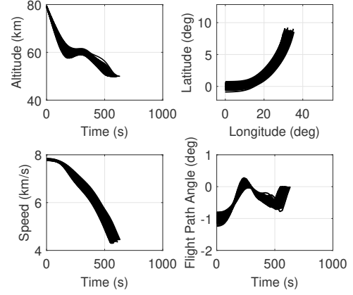
Fig. 8: 500 evolutions of the state results
