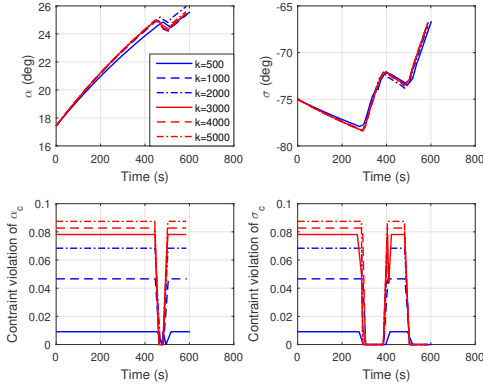
Fig. 7: Sensitivity results with respect to k
