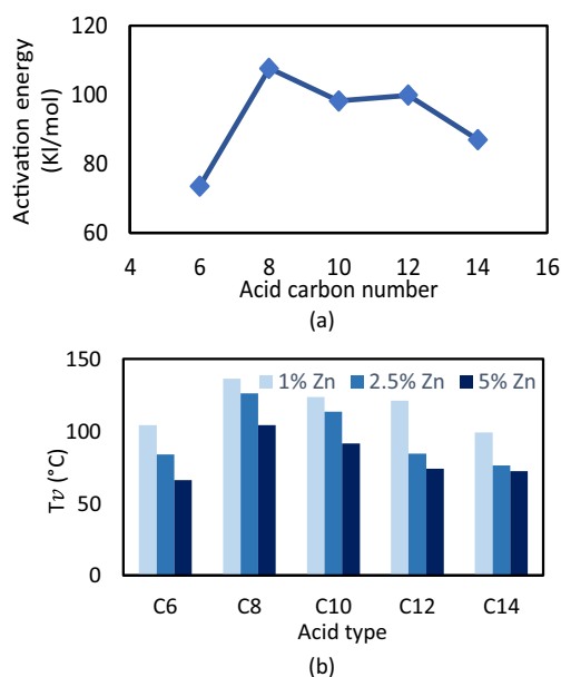
FIGURE 4 Activation energy (a) and topology freezing temperature; (b) for all vitrimer formulations as a function of chain length. [Color figure can be viewed at wileyonlinelibrary.com ]
