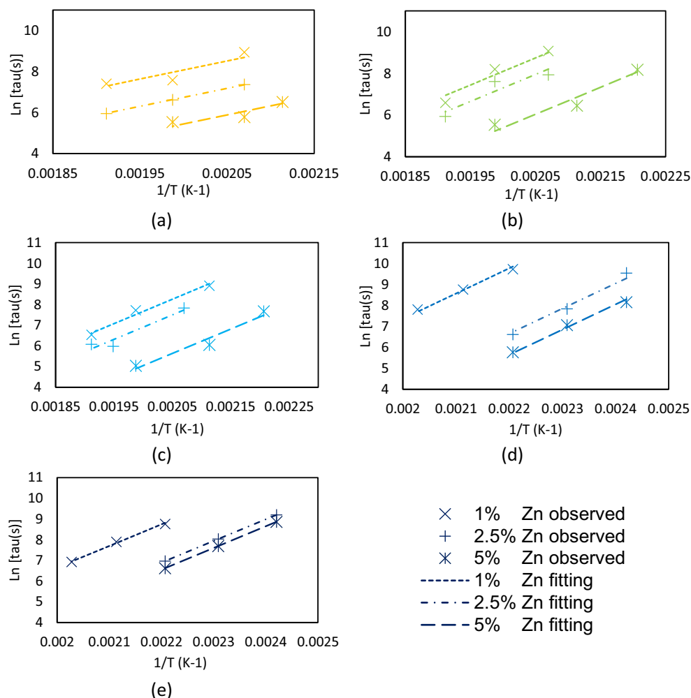
FIGURE 3 Stress relaxation Arrhenius fitting: (a) C6; (b) C8; (c) C10; (d) C12; (e) C14. [Color figure can be viewed at wileyonlinelibrary.com ]
