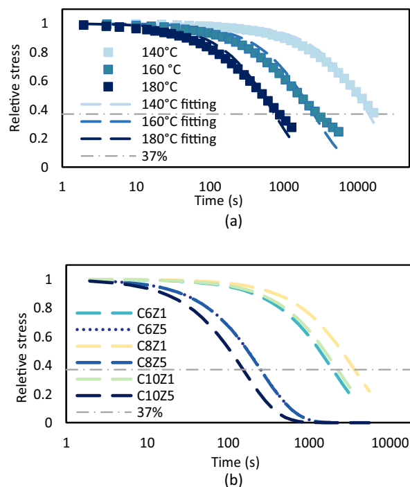
FIGURE 2 Normalized stress relaxation curves of (a) dodecanedioic acid vitrimer with 2.5% catalyst at 140, 160 and 180°C; (b) adipic, suberic and sebacic acid formulations at 230°C. [Color figure can be viewed at wileyonlinelibrary.com ]
