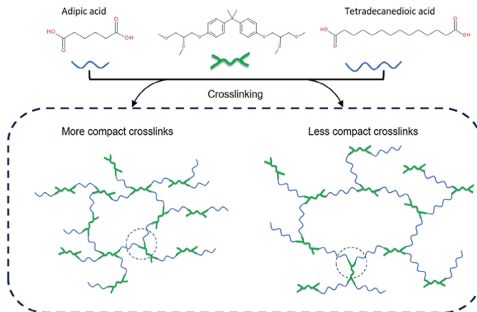
FIGURE 6 Difference in the crosslinked structure of vitrimer made of linear dicarboxylic acid with varied number of methylene groups. [Color figure can be viewed at wileyonlinelibrary.com ]
