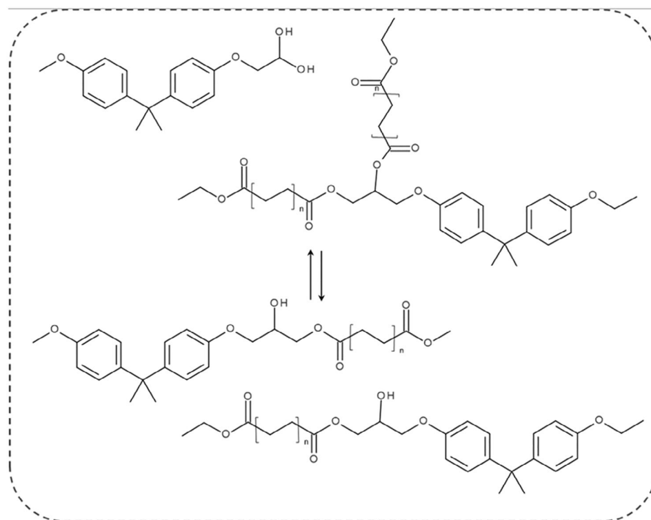
FIGURE 5 Exchange process via transesterification in hydroxy-ester networks.
