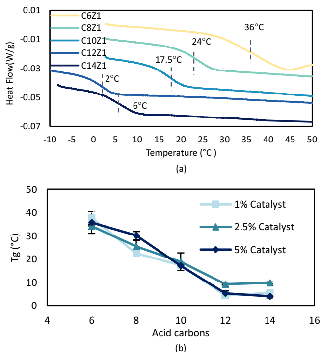
FIGURE 7 (a) DSC results and (b) glass transition temperature of vitrimers with different carboxylic acids. [Color figure can be viewed at wileyonlinelibrary.com ]
