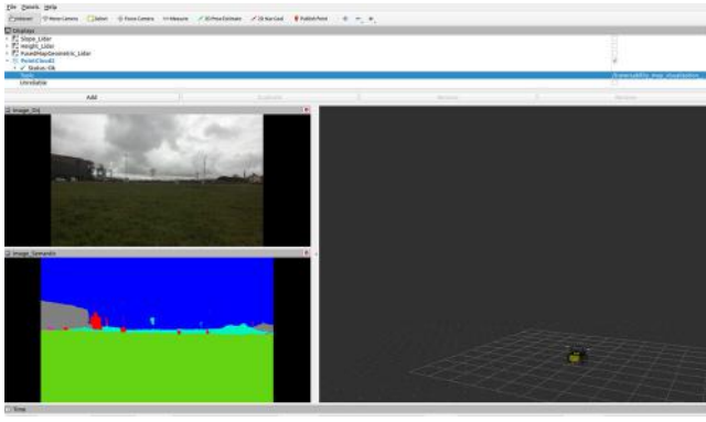
FIGURE 9 | Real-time semantic segmentation-based terrain classification and traversability cloud for representing the semantic segmentation model to 2.5D map. [Color figure can be viewed at wileyonlinelibrary.com ]
