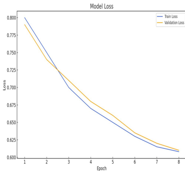
Fig. 22 ResNet50 loss
