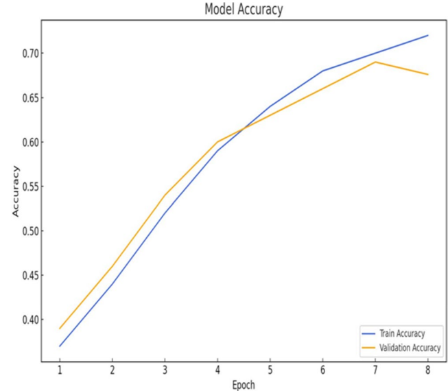
Fig. 21 ResNet50 accuracy
