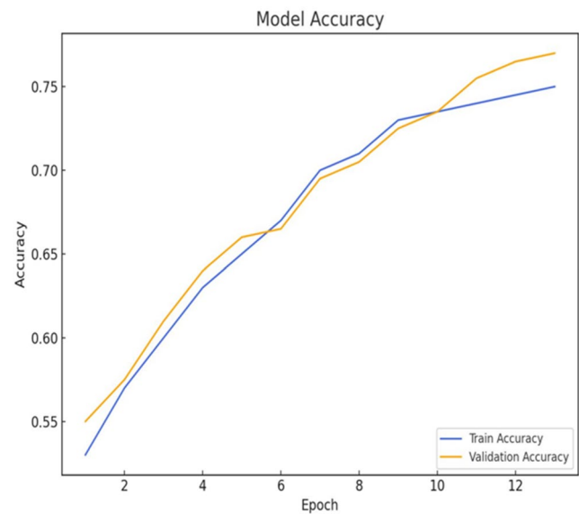
Fig. 24 MobileNet accuracy
