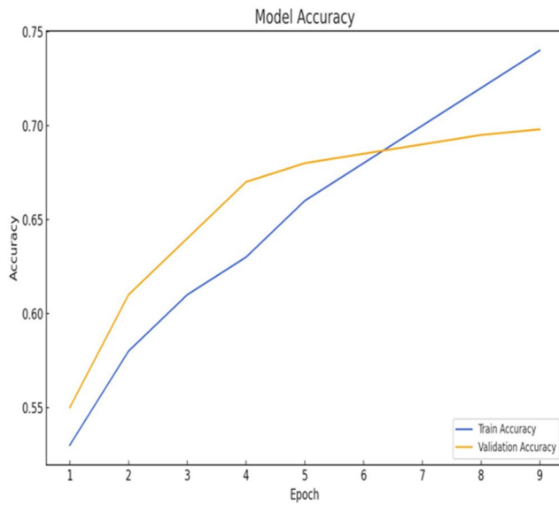
Fig. 18 EfficientNetB0 accuracy
