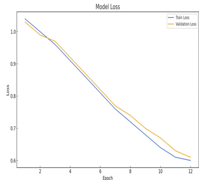
Fig. 25 MobileNet loss
