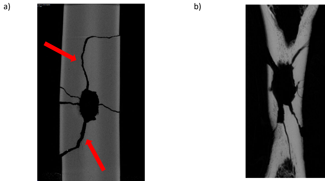
Fig 8 A comparison CT scan of the a) generic cylinder and b) porcine bone to observe the fracture patterns and pore structure
