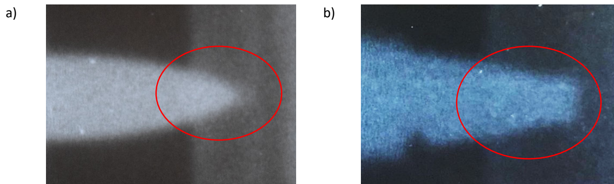
Fig 12 X-rays of the reverse ballistic targets, each identifying the conical region of compressed pores.
