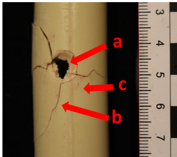
Fig 7 A generic cylinder target; embedded in ballistic gel and impacted with a steel ball. a) the depressed ring; b) a primary fracture; c) a secondary fracture
