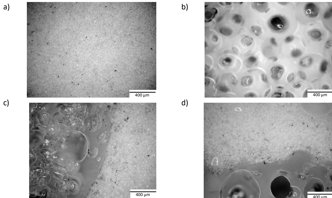
Fig 1 Light microscopy images of four types of Synbone®. a) generic cylinder; b) osteoporotic cylinder; c) humerus model; d) femur model
