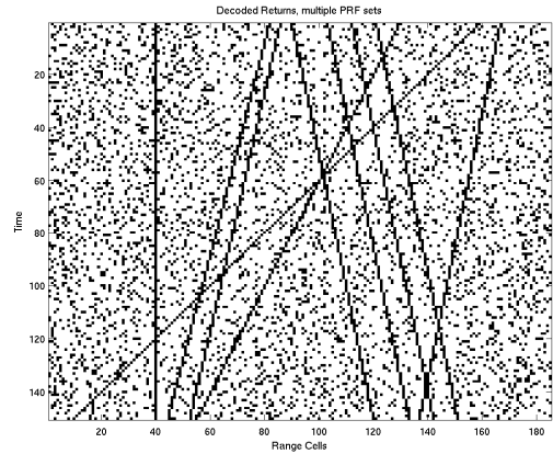
Figure 2. Effect of Scan to Scan PRI Change
