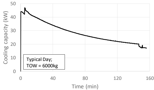
Figure 15: Fuel System cooling capacity throughout the PAT mission
