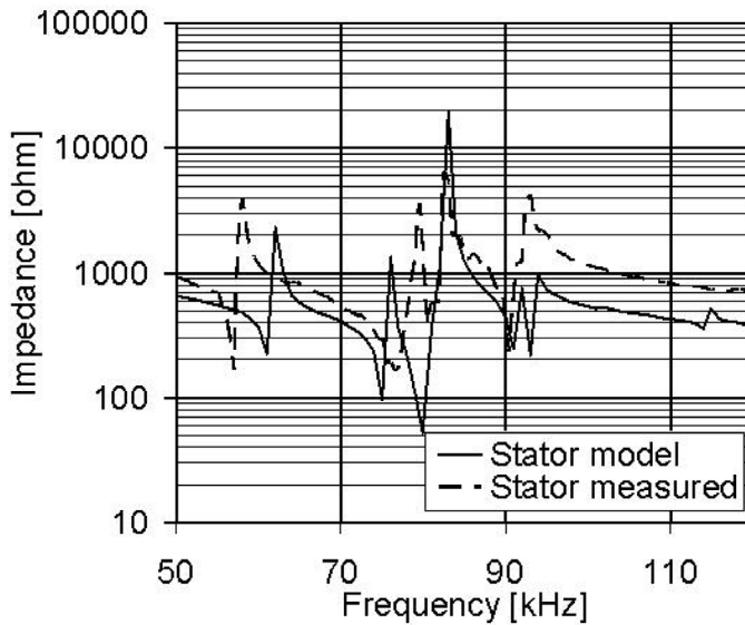
Fig. 6. Modeled and measured impedance characteristics of the complete stator structure (cymbal+PZT plate).
