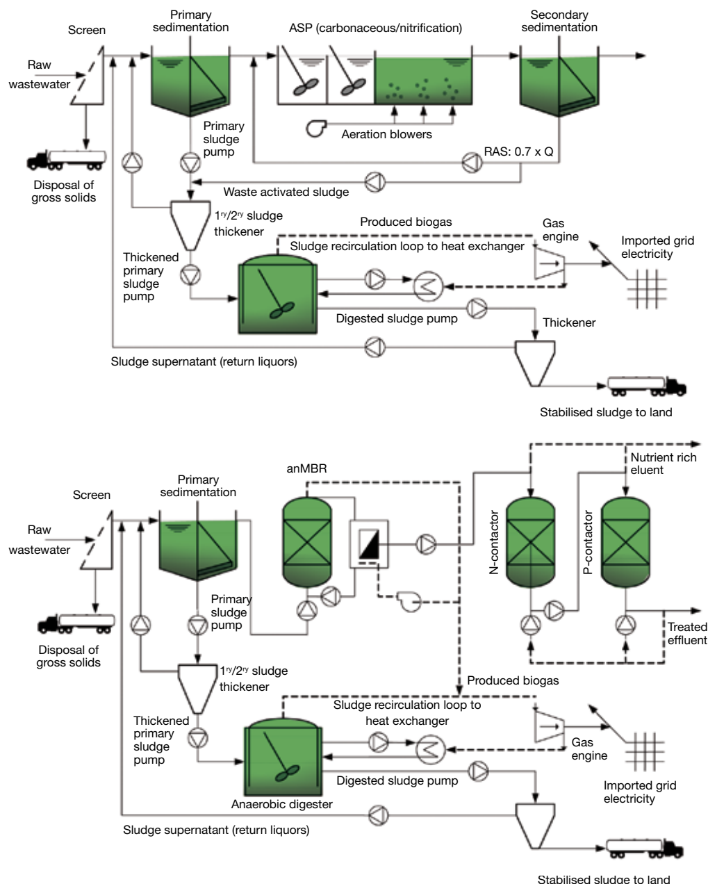
Figure 1: Conventional wastewater flowsheet comprising an aerated activated sludge process (top) versus an alternate flowsheet proposed by Cranfield comprising anMBR followed by physico-chemical recovery of ammonia and phosphorus (bottom).
