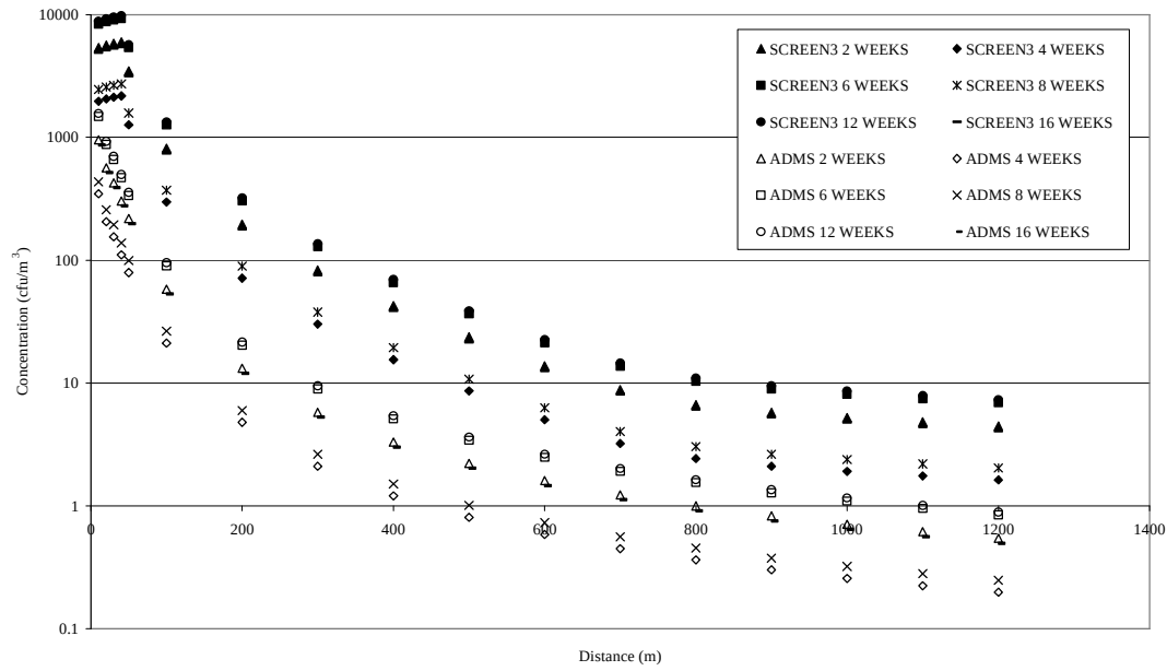
Fig 5. Source depletion curves of actinomycetes from passive emissions estimated using the SCREEN3 and ADMS dispersion models
