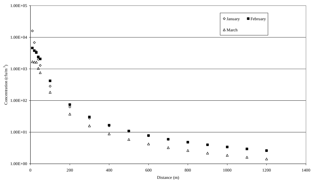
Fig 11. Estimated depletion curves of actinomycetes using the ADMS model for combined active and passive sources on three separate dates.
