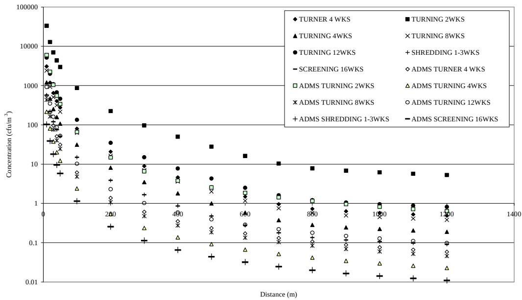
Fig 6. Source depletion curves of Aspergillus fumigatus from agitation activities estimated using the SCREEN3 and ADMS dispersion models
