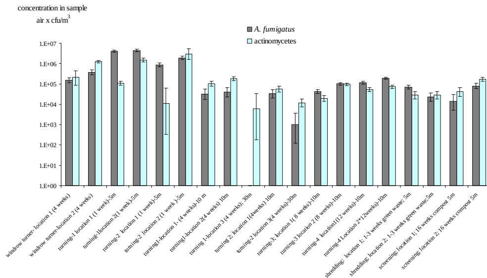
Fig. 3. Bioaerosols concentration at 5m, 10m and 30m measured while agitation activities were taking place
