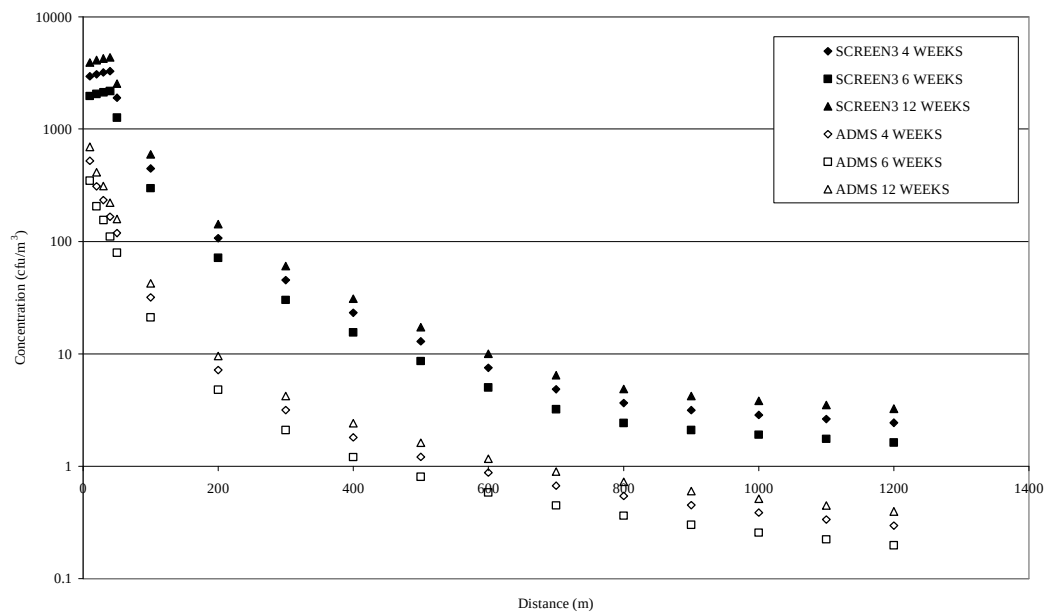
Fig 4. Source depletion curves of Aspergillus fumigatus from passive emissions estimated using the SCREEN3 and ADMS dispersion models
