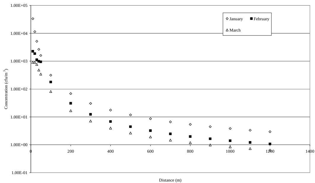
Fig 10. Estimated depletion curves of Aspergillus fumigatus using the ADMS model for combined active and passive sources on three separate dates.
