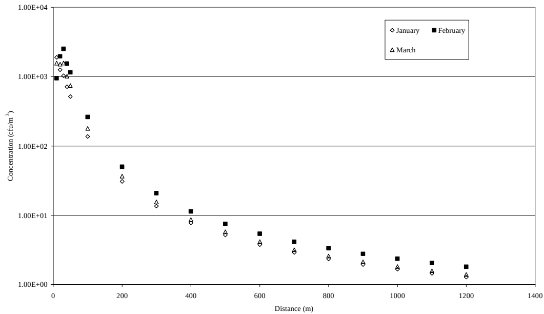
Fig 9. Estimated depletion curves of actinomycetes using the ADMS model for combined passive sources on three separate dates.
