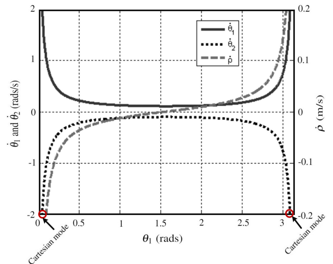
FIGURE 2. Behaviour of joint velocities at input cartesian speed of 0.02\text{ m/s} in horizontal tracking.
