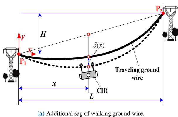
FIGURE 3. Cables subject to additional sag with function, \delta(x) due to additional weight of climbing robot. To express the sag various factors are taken into considered: suspension points (i.e. P_1 and P_2 ) on tower, cross-sectional area of cables, L as horizontal spacing, horizontal stress of power line, and impact effect. This impact effect represents vibrations from robot and wind (left) and robot on double 315-kV circuits (right) [47].
