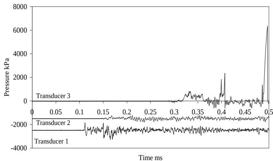
Figure 6 The initial part of the data from Figure 5 showing the staggered pressure wave arrival at each transducer.
