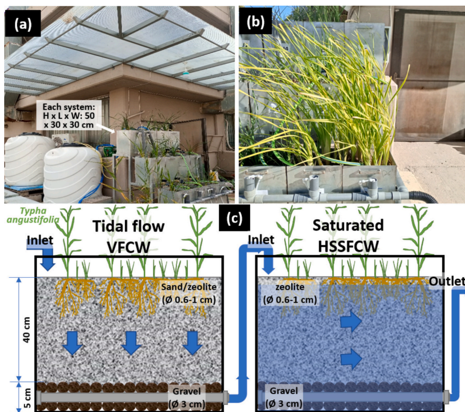
Fig. 1. The photo of the mesocosm-scale hybrid constructed wetland systems (CWs) set up at the beginning (a) and at the middle period (b) of the study. The schematic of each hybrid system (c) consisted of a tidal flow CW and a saturated horizontal flow CW.
