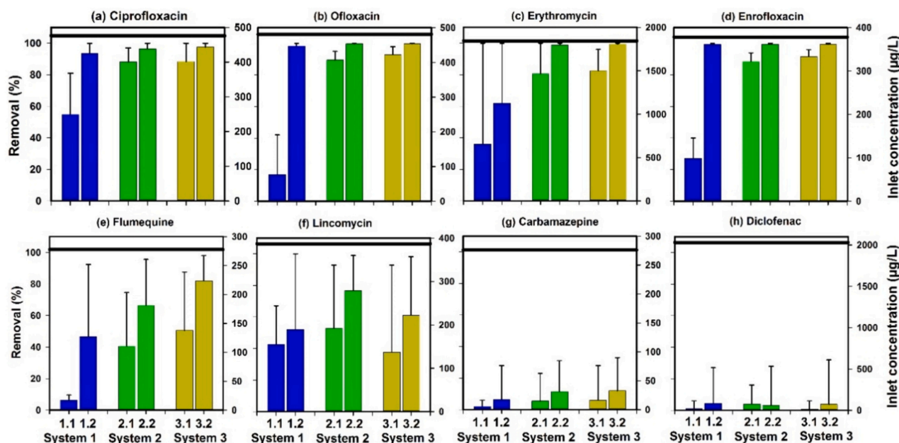
Fig. 3. The average influent concentrations (lines) and the removal efficiencies (bars) of pharmaceuticals, including ciprofloxacin (a), ofloxacin (b), erythromycin (c), enrofloxacin (d) flumequine (e), lincomycin (f), carbamazepine (g), and diclofenac (h), in each hybrid constructed wetland (CW). System 1.1, 2.1, and 3.1 represent tidal flow CWs filled with sand, raw zeolite, and modified zeolite, respectively. System 1.2, 2.2, and 3.2 indicate horizontal subsurface flow CWs filled with raw zeolite. Blue, green, and yellow bars represent the results from system 1, 2, and 3, respectively.
