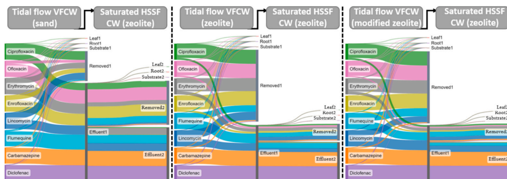
Fig. 4. Sankey diagram of the mass distribution for pharmaceutical compounds at three hybrid CWs.
