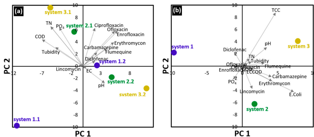
Fig. 5. Principal component analysis (PCA) of the treatment performance patterns in each constructed wetland (CW) system (a) and the overall performance of three hybrid CWs (b). The original data used for the factors (arrows in the figure) were the value differences between influent and effluent (removal efficiencies).
