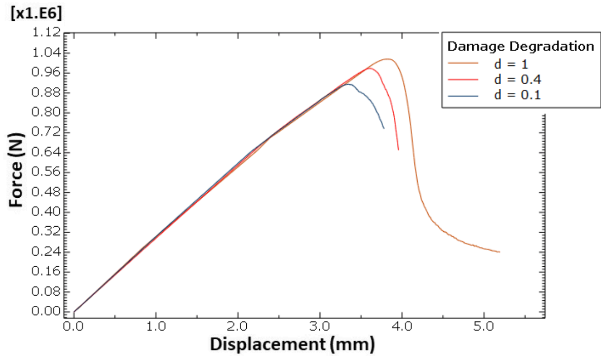
Figure 17: Force - Displacement diagrams for position B with damage degradation coefficient equal to 0.1, 0.4 & 1
