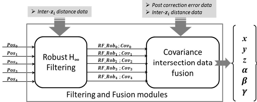
Figure 3. Filtering modules
