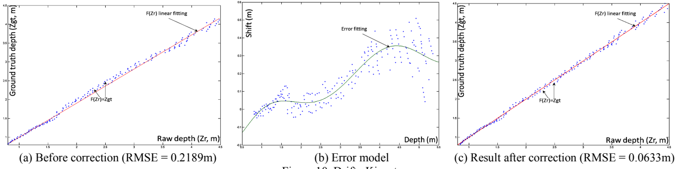
Figure 10. Drifty Kinect
