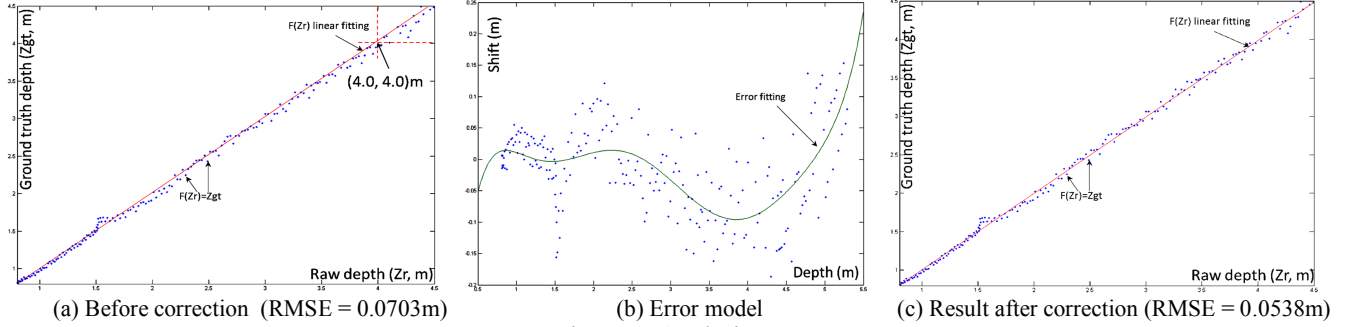
Figure 11. Good Kinect
