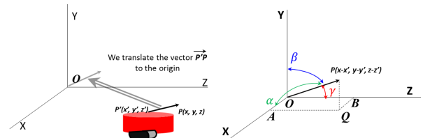
(c) Pose of the robot in the scene (d) Orientation definition Figure 7. Orientation computation.
