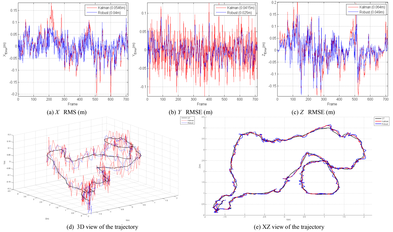
Figure 13. The best tracking results after applying Robust H_\infty and Kalman filters on X,Y and Z coordinates
