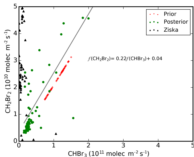
Figure 5. Scatterplot between \text{CHBr}_3 and \text{CH}_2\text{Br}_2 fluxes described on 2^\circ (latitude) \times 2.5^\circ (longitude) grid boxes over the main study region ( 130\text{--}155^\circ\text{E} and 0\text{--}12^\circ\text{N} , Fig. 1). Red crosses denote values from Ordóñez et al. (2012), which we use for our a priori; black triangles denote values from an alternative bottom-up inventory (Ziska et al., 2013); and green circles denote our a posteriori values. A posteriori fluxes of \text{CHBr}_3 and \text{CH}_2\text{Br}_2 have a Pearson correlation of 0.86, and the best-fit linear model for the a posteriori fluxes is shown inset.
