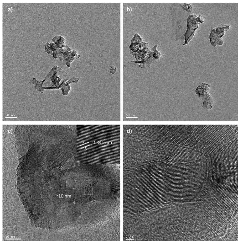
Fig. 8. Representative HR-TEM images of the nano carbon sample NC HT2 , showing the general morphology of the samples at lower magnification a,b (scale bar 50 nm) and the graphitic nature with higher magnification c,d (scale bar 10 and 2 nm) allowing the identification of ordered domains within the samples.
