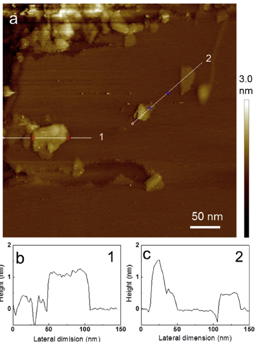
Fig. 7. (a) Ambient STM image of deposits of nano carbon dispersion ( \text{NC}_{\text{HT2}} ) on freshly cleaved HOPG surface. Several individual nano carbons and some nano carbon aggregations (top) are clearly seen. (b, c) Cross sections taken along the white lines 1 and 2. (A colour version of this figure can be viewed online.)
